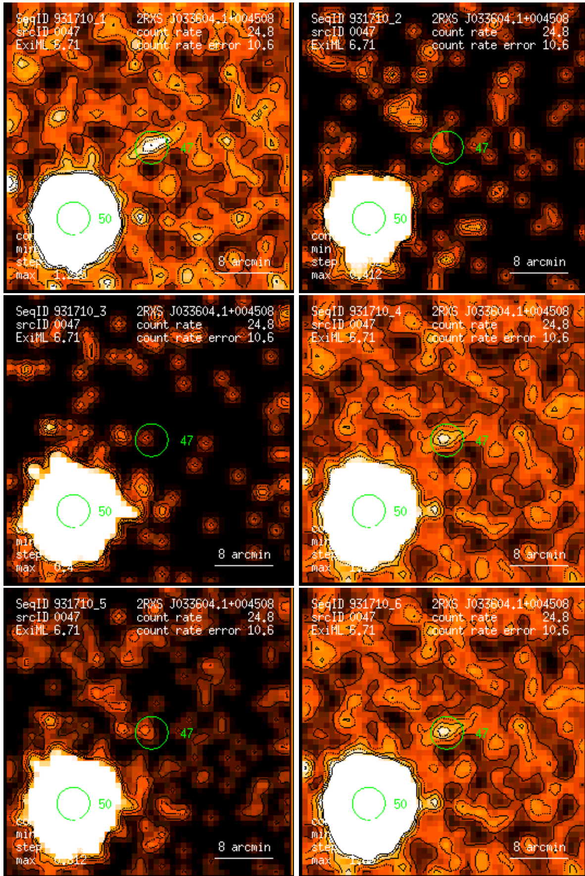
Figure 47: RASS 931710: detection 0047: band rate images, Gaussian filter: (1) PSPC channels 11 – 41, (2) 52 – 90, (3) 91 – 201, (4) 11 – 235, (5) 52 – 201, (6) 11 – 201. Broad band rates in counts/ks. Band rate contour levels in counts/ks/arcmin 2 .
