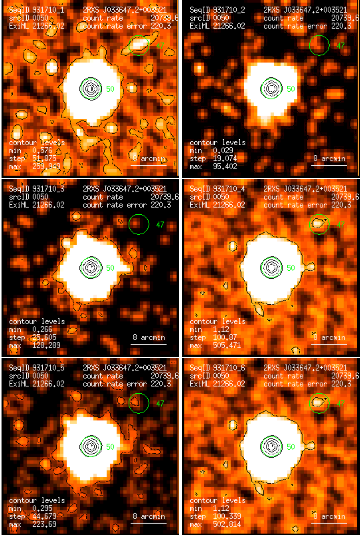
Figure 50: RASS 931710: detection 0050: band rate images, Gaussian filter: (1) PSPC channels 11 – 41, (2) 52 – 90, (3) 91 – 201, (4) 11 – 235, (5) 52 – 201, (6) 11 – 201. Broad band rates in counts/ks. Band rate contour levels in counts/ks/arcmin 2 .
