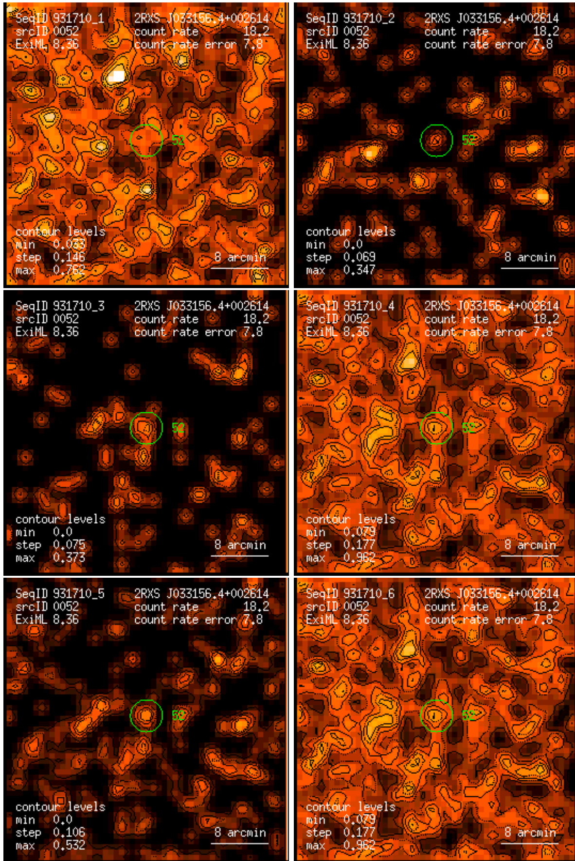
Figure 52: RASS 931710: detection 0052: band rate images, Gaussian filter: (1) PSPC channels 11 – 41, (2) 52 – 90, (3) 91 – 201, (4) 11 – 235, (5) 52 – 201, (6) 11 – 201. Broad band rates in counts/ks. Band rate contour levels in counts/ks/arcmin 2 .
