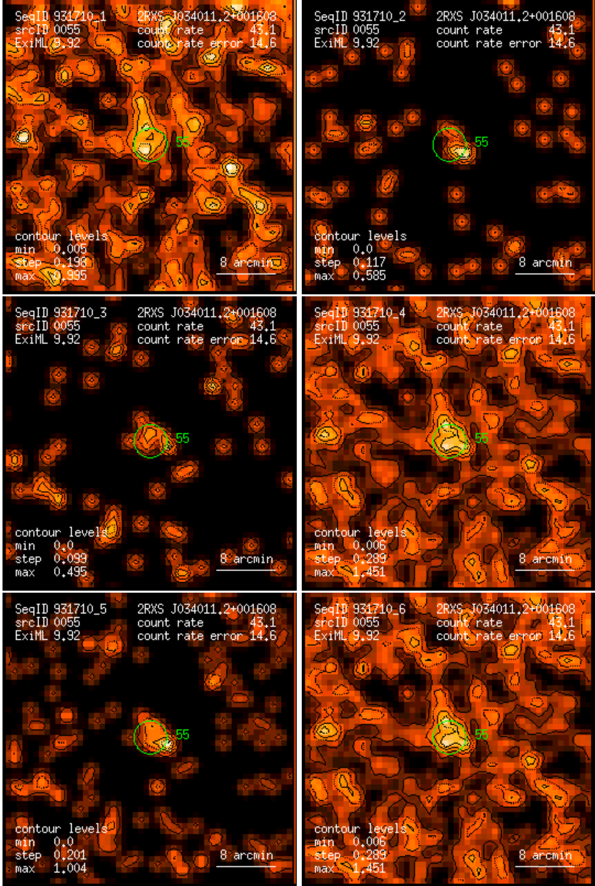
Figure 55: RASS 931710: detection 0055: band rate images, Gaussian filter: (1) PSPC channels 11 – 41, (2) 52 – 90, (3) 91 – 201, (4) 11 – 235, (5) 52 – 201, (6) 11 – 201. Broad band rates in counts/ks. Band rate contour levels in counts/ks/arcmin 2 .
