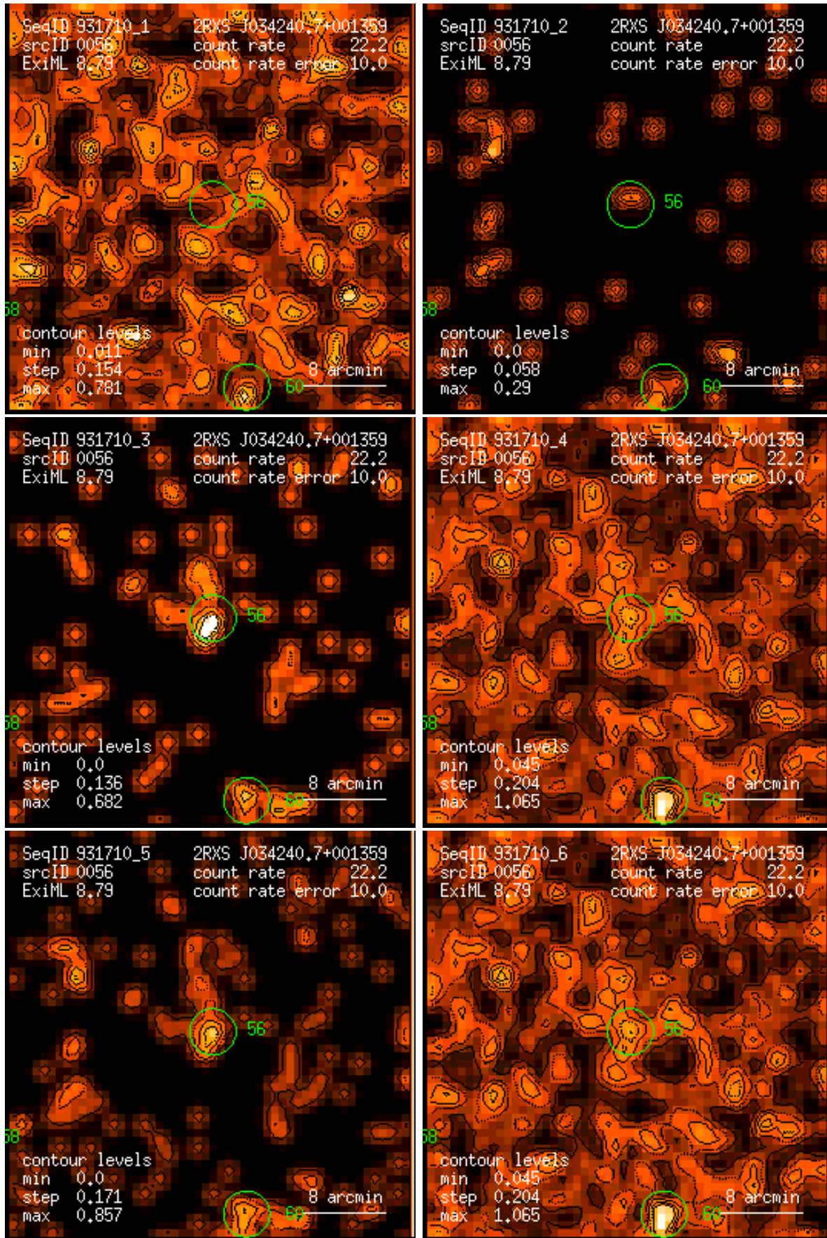
Figure 56: RASS 931710: detection 0056: band rate images, Gaussian filter: (1) PSPC channels 11 – 41, (2) 52 – 90, (3) 91 – 201, (4) 11 – 235, (5) 52 – 201, (6) 11 – 201. Broad band rates in counts/ks. Band rate contour levels in counts/ks/arcmin 2 .
