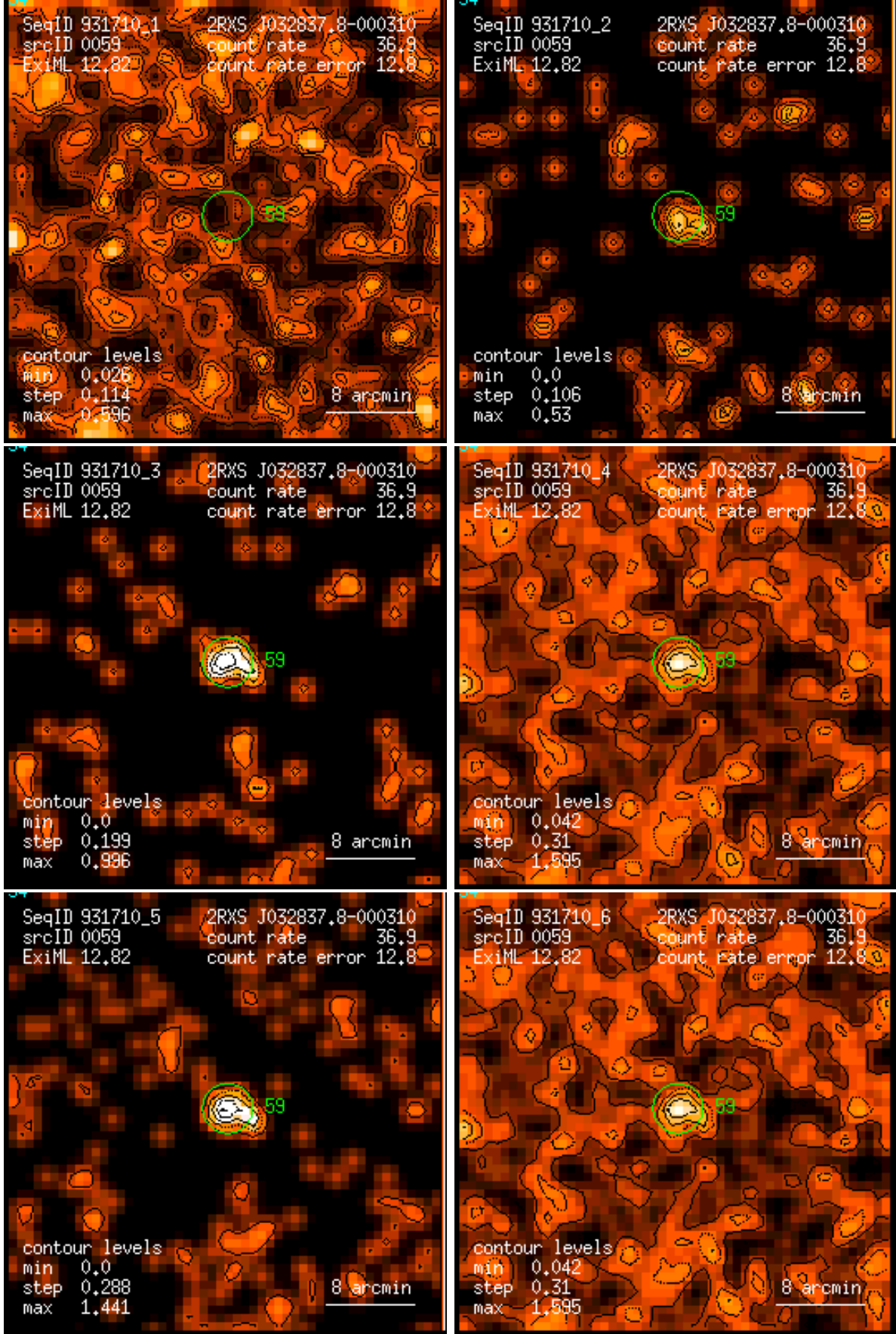
Figure 59: RASS 931710: detection 0059: band rate images, Gaussian filter: (1) PSPC channels 11 – 41, (2) 52 – 90, (3) 91 – 201, (4) 11 – 235, (5) 52 – 201, (6) 11 – 201. Broad band rates in counts/ks. Band rate contour levels in counts/ks/arcmin 2 .
