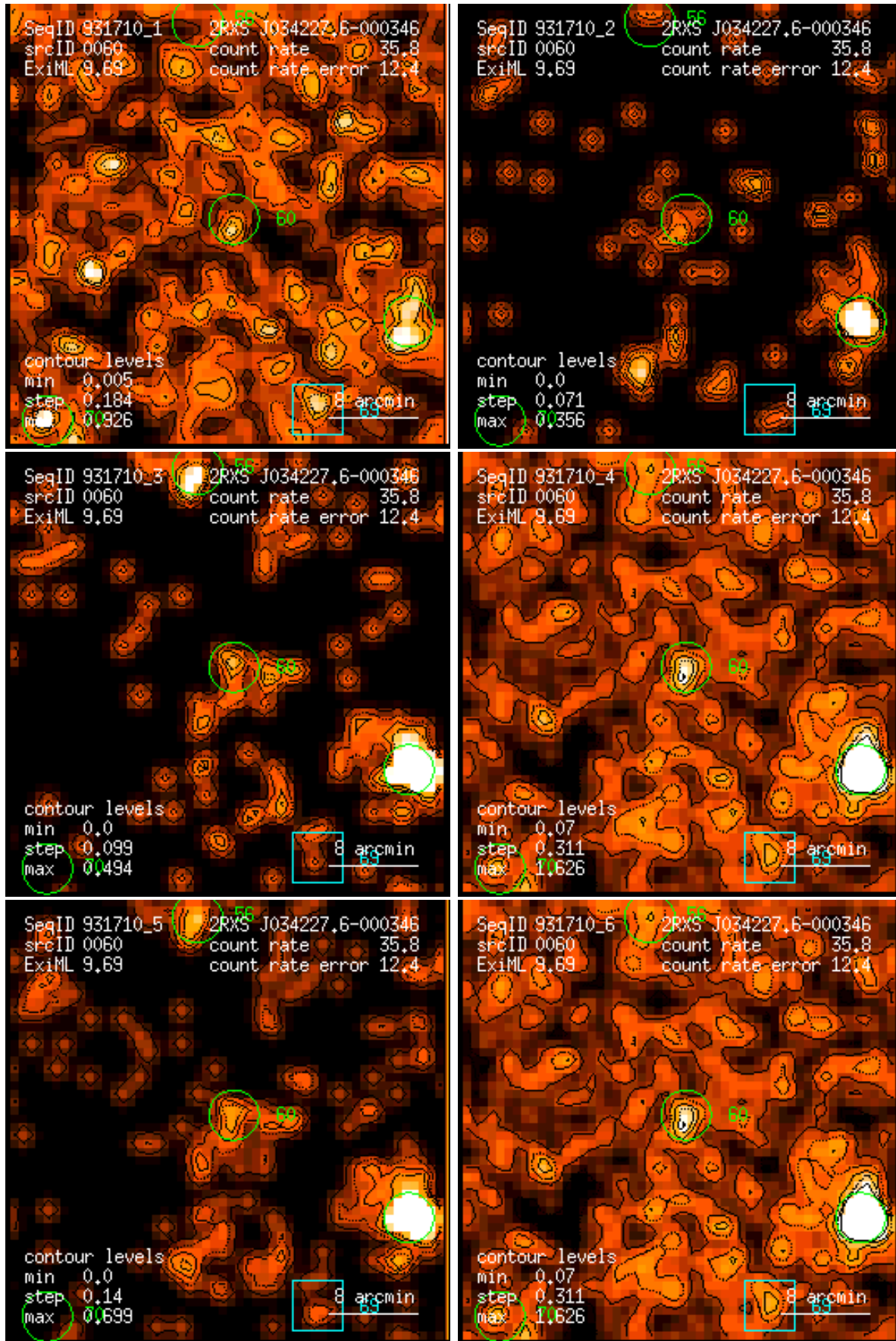
Figure 60: RASS 931710: detection 0060: band rate images, Gaussian filter: (1) PSPC channels 11 – 41, (2) 52 – 90, (3) 91 – 201, (4) 11 – 235, (5) 52 – 201, (6) 11 – 201. Broad band rates in counts/ks. Band rate contour levels in counts/ks/arcmin 2 .
