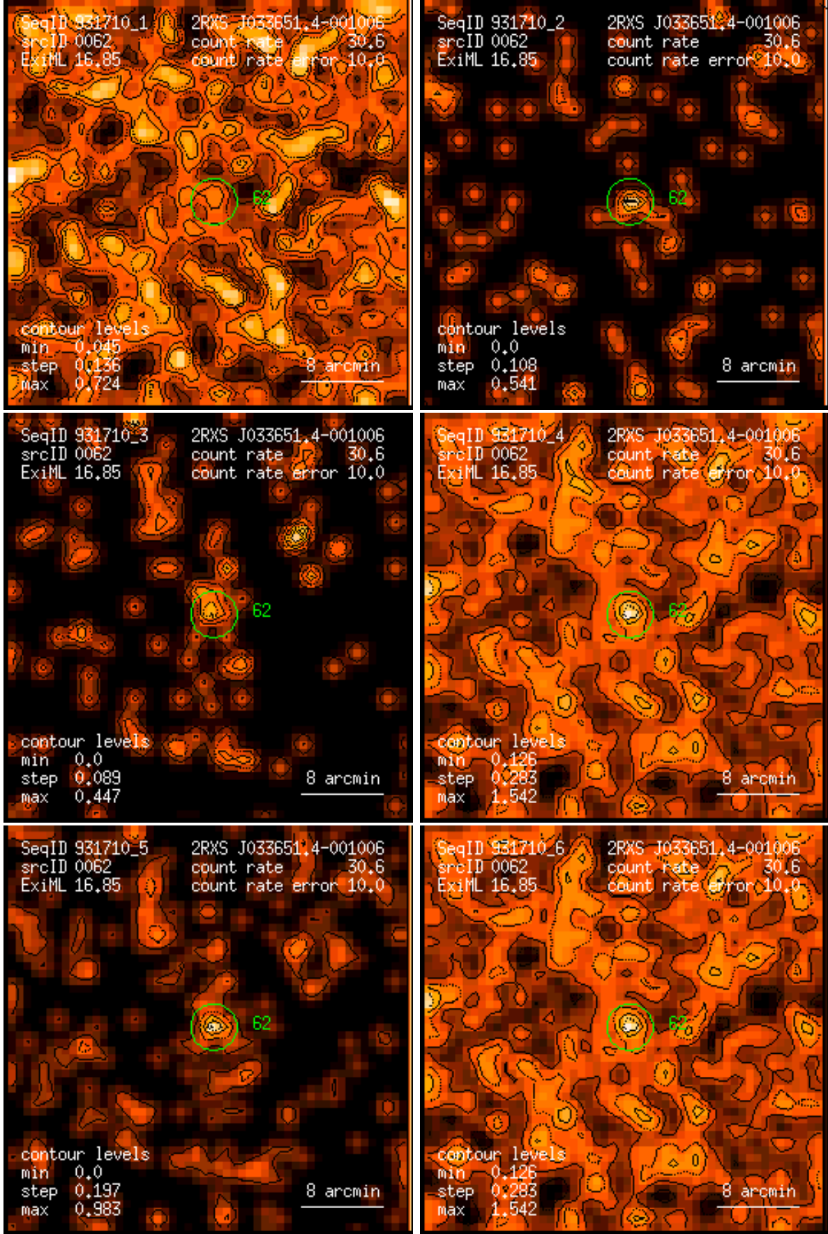
Figure 62: RASS 931710: detection 0062: band rate images, Gaussian filter: (1) PSPC channels 11 – 41, (2) 52 – 90, (3) 91 – 201, (4) 11 – 235, (5) 52 – 201, (6) 11 – 201. Broad band rates in counts/ks. Band rate contour levels in counts/ks/arcmin 2 .
