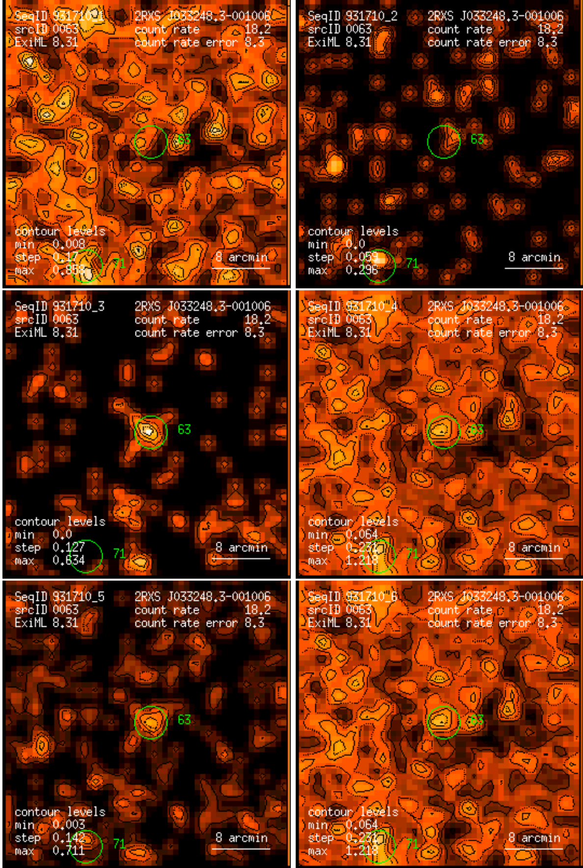
Figure 63: RASS 931710: detection 0063: band rate images, Gaussian filter: (1) PSPC channels 11 – 41, (2) 52 – 90, (3) 91 – 201, (4) 11 – 235, (5) 52 – 201, (6) 11 – 201. Broad band rates in counts/ks. Band rate contour levels in counts/ks/arcmin 2 .
