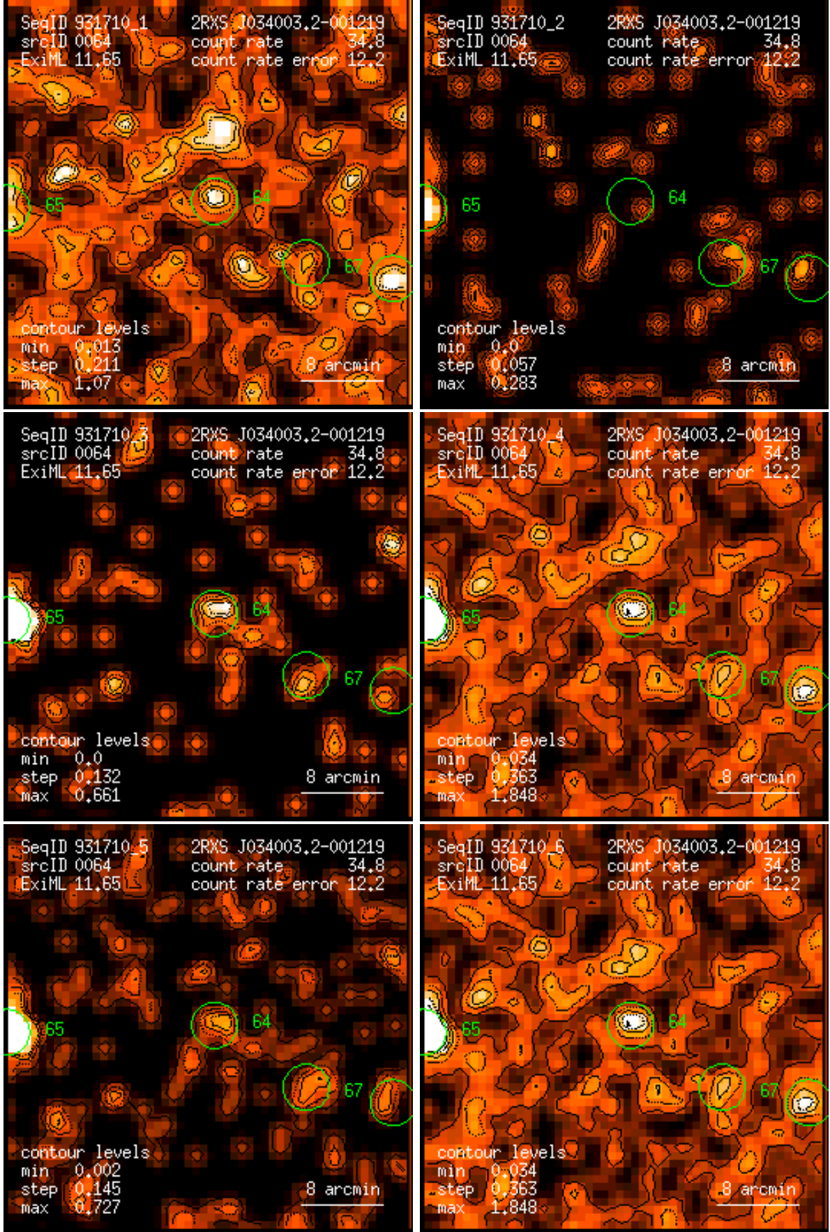
Figure 64: RASS 931710: detection 0064: band rate images, Gaussian filter: (1) PSPC channels 11 – 41, (2) 52 – 90, (3) 91 – 201, (4) 11 – 235, (5) 52 – 201, (6) 11 – 201. Broad band rates in counts/ks. Band rate contour levels in counts/ks/arcmin 2 .
