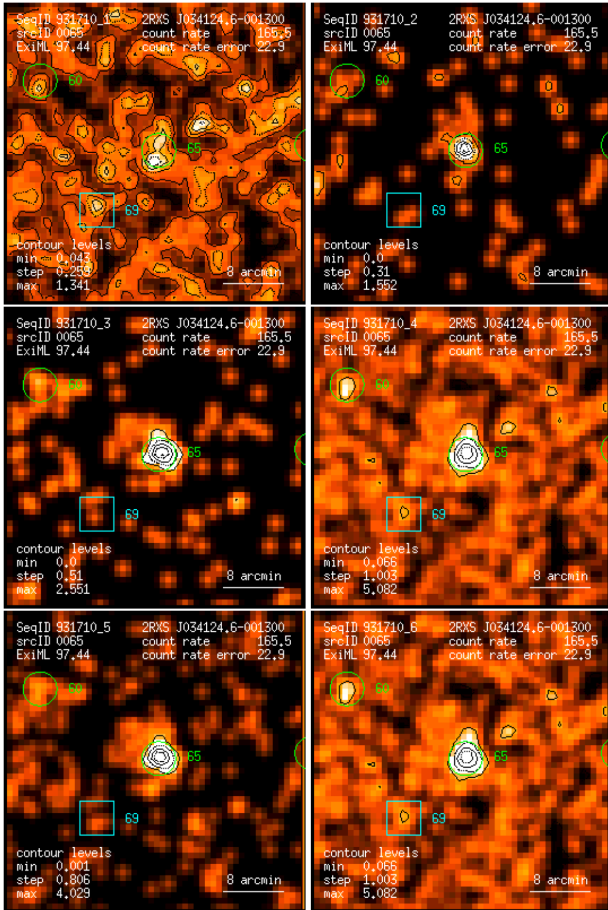
Figure 65: RASS 931710: detection 0065: band rate images, Gaussian filter: (1) PSPC channels 11 – 41, (2) 52 – 90, (3) 91 – 201, (4) 11 – 235, (5) 52 – 201, (6) 11 – 201. Broad band rates in counts/ks. Band rate contour levels in counts/ks/arcmin 2 .
