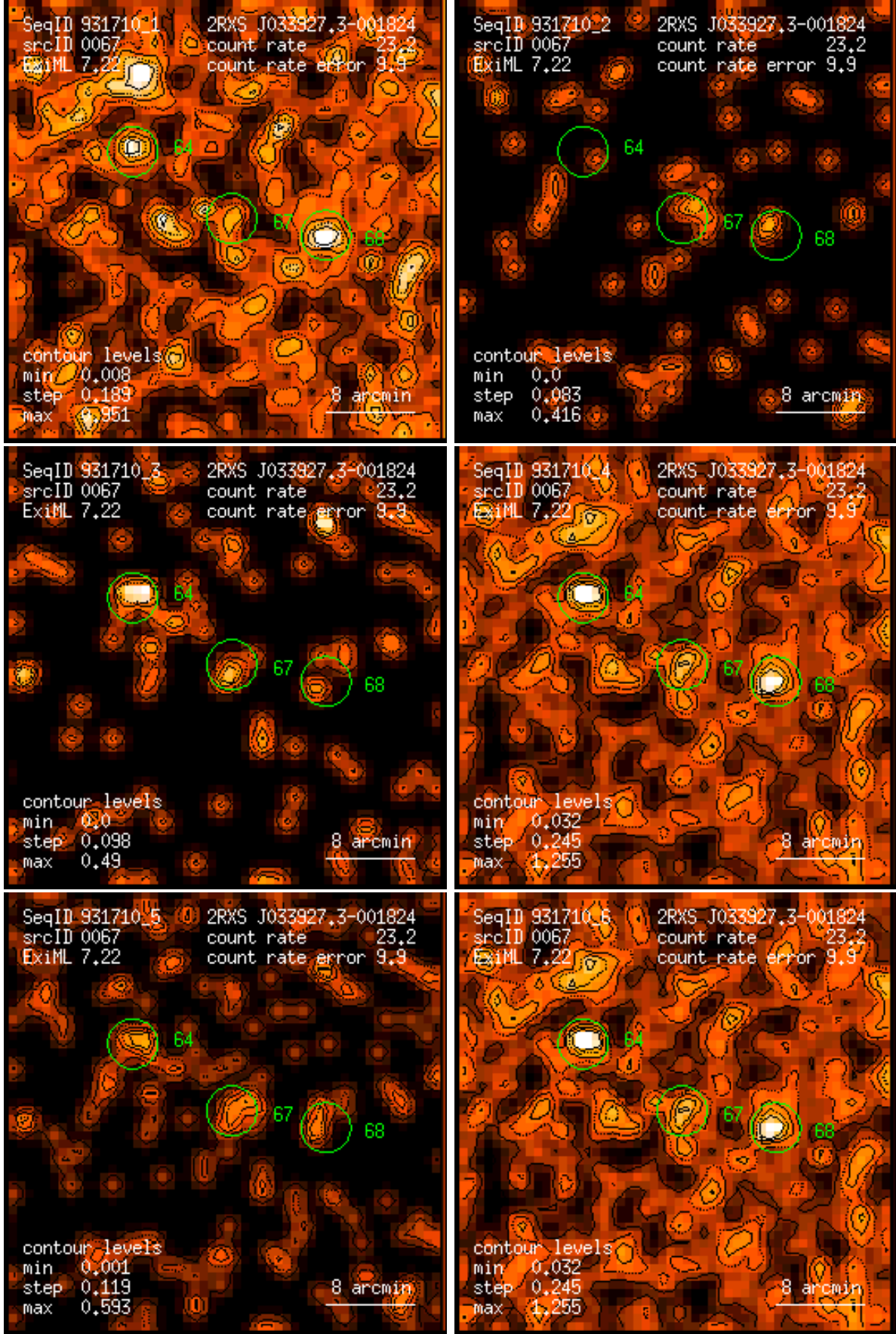
Figure 67: RASS 931710: detection 0067: band rate images, Gaussian filter: (1) PSPC channels 11 – 41, (2) 52 – 90, (3) 91 – 201, (4) 11 – 235, (5) 52 – 201, (6) 11 – 201. Broad band rates in counts/ks. Band rate contour levels in counts/ks/arcmin 2 .
