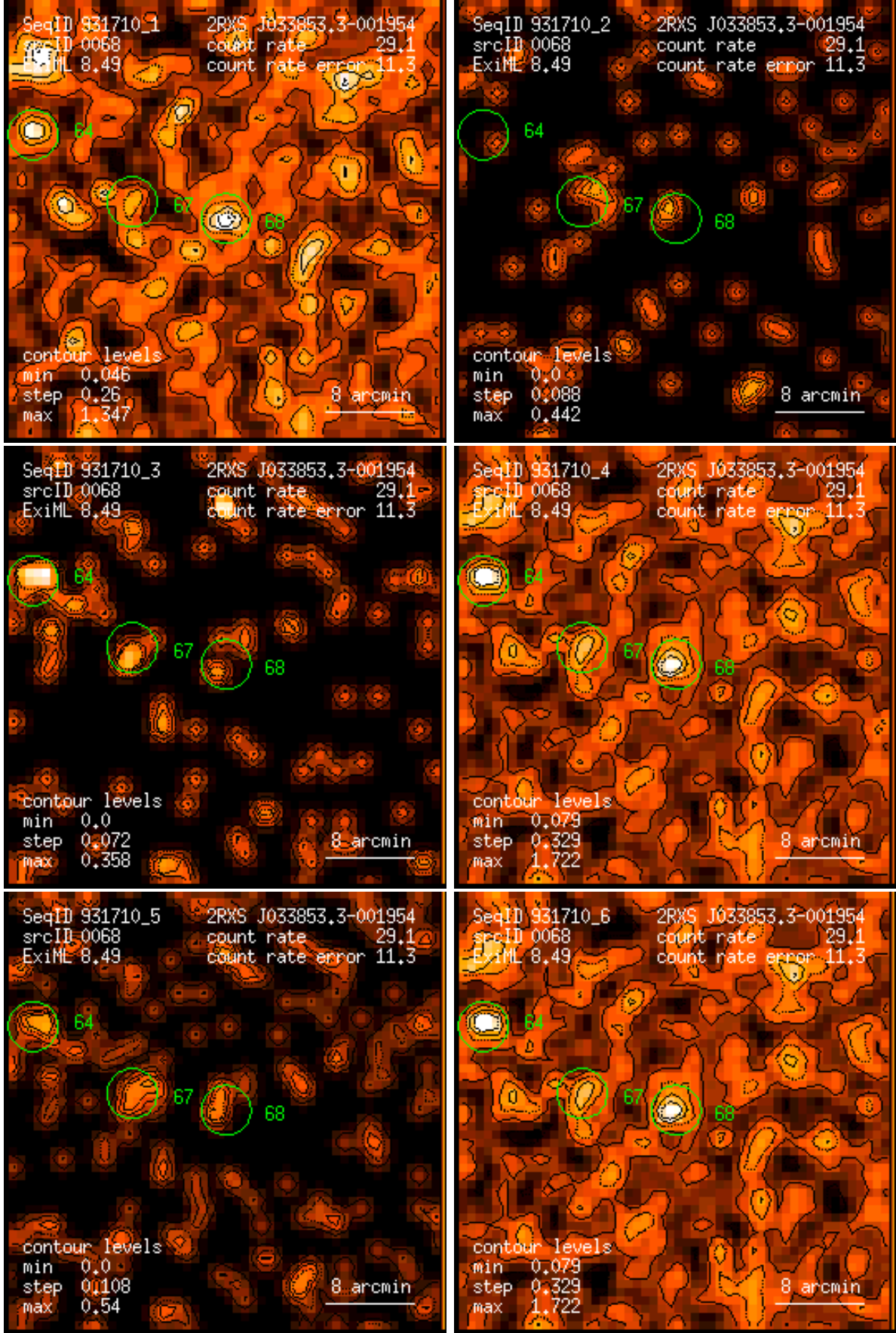
Figure 68: RASS 931710: detection 0068: band rate images, Gaussian filter: (1) PSPC channels 11 – 41, (2) 52 – 90, (3) 91 – 201, (4) 11 – 235, (5) 52 – 201, (6) 11 – 201. Broad band rates in counts/ks. Band rate contour levels in counts/ks/arcmin 2 .
