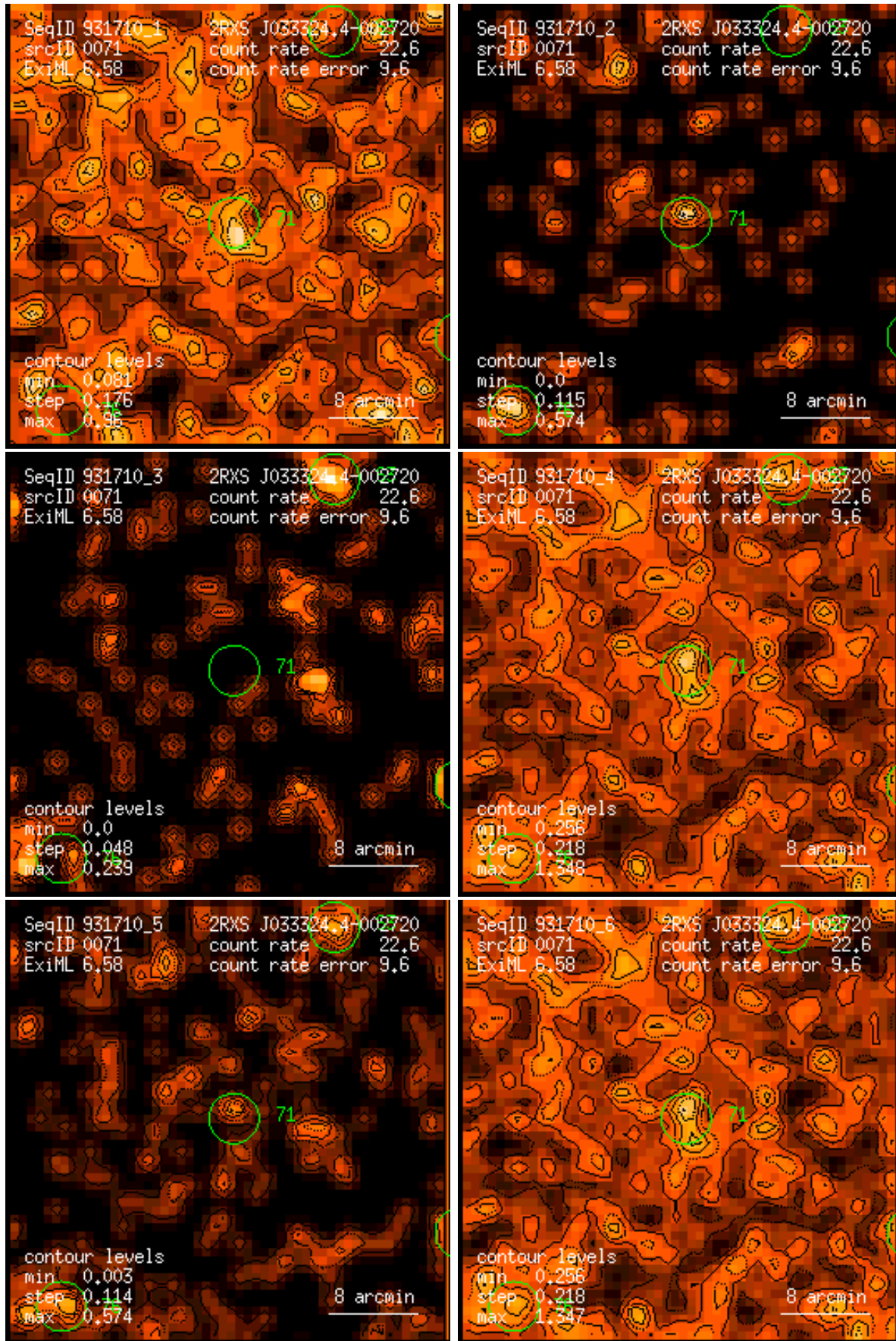
Figure 71: RASS 931710: detection 0071: band rate images, Gaussian filter: (1) PSPC channels 11 – 41, (2) 52 – 90, (3) 91 – 201, (4) 11 – 235, (5) 52 – 201, (6) 11 – 201. Broad band rates in counts/ks. Band rate contour levels in counts/ks/arcmin 2 .
