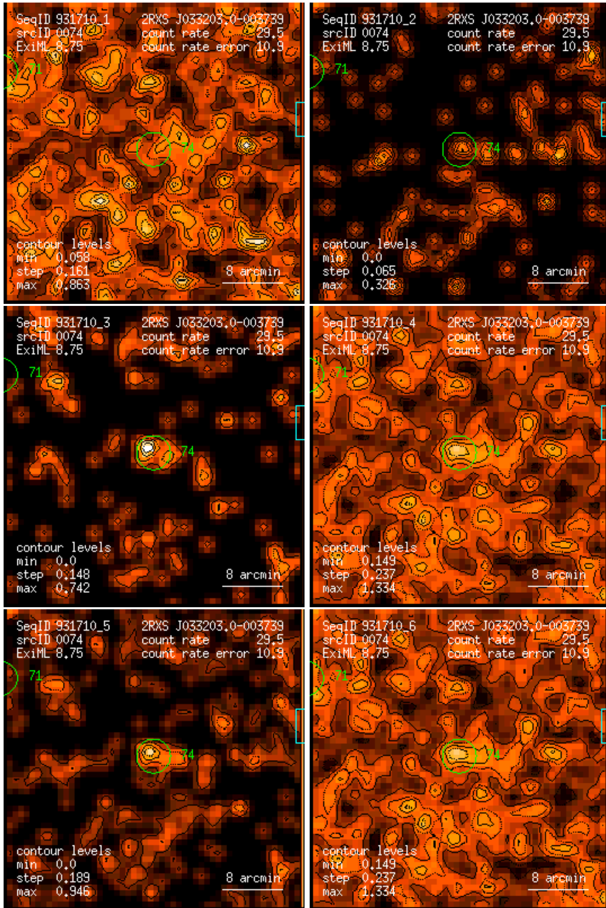
Figure 74: RASS 931710: detection 0074: band rate images, Gaussian filter: (1) PSPC channels 11 – 41, (2) 52 – 90, (3) 91 – 201, (4) 11 – 235, (5) 52 – 201, (6) 11 – 201. Broad band rates in counts/ks. Band rate contour levels in counts/ks/arcmin 2 .
