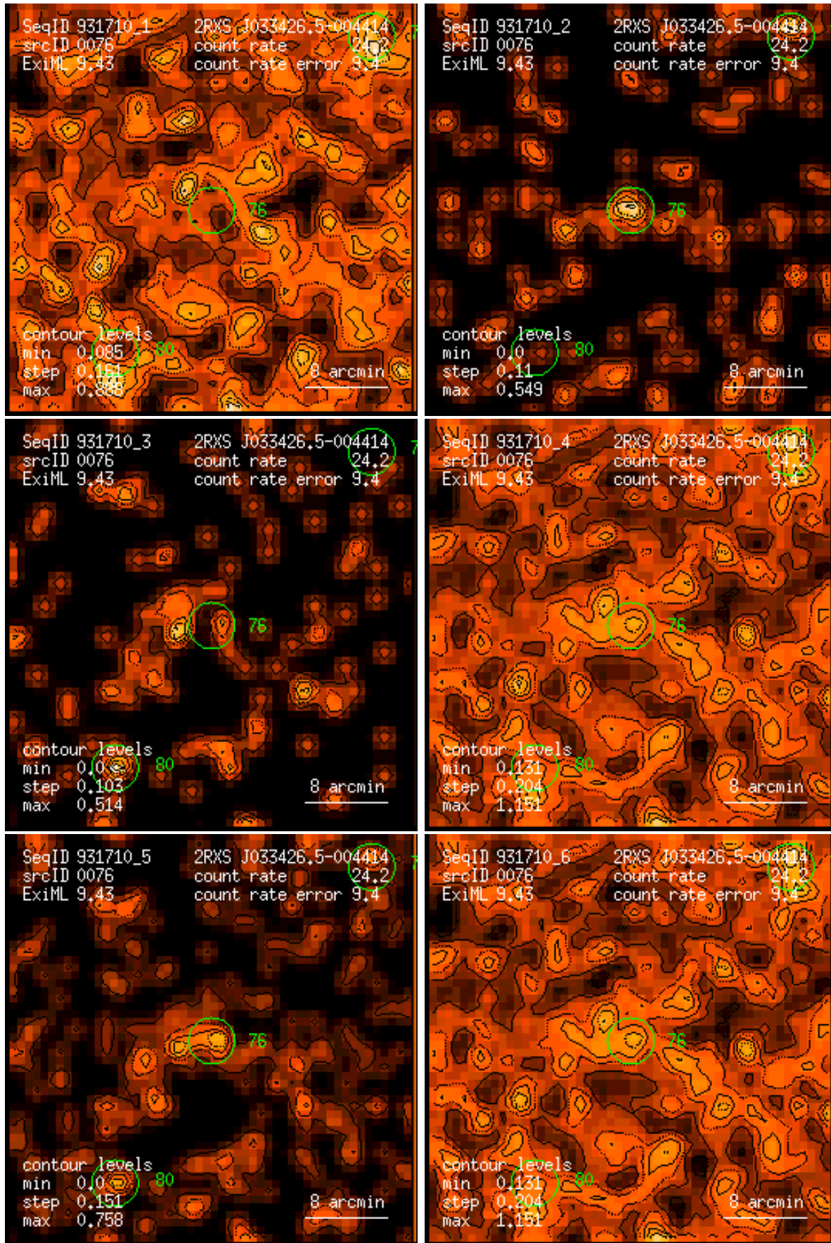
Figure 76: RASS 931710: detection 0076: band rate images, Gaussian filter: (1) PSPC channels 11 – 41, (2) 52 – 90, (3) 91 – 201, (4) 11 – 235, (5) 52 – 201, (6) 11 – 201. Broad band rates in counts/ks. Band rate contour levels in counts/ks/arcmin 2 .
