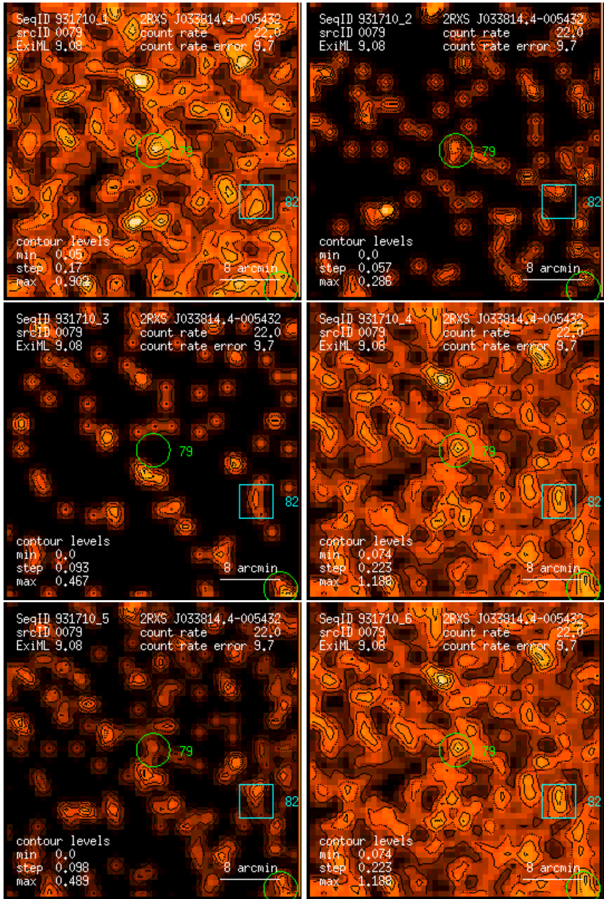
Figure 79: RASS 931710: detection 0079: band rate images, Gaussian filter: (1) PSPC channels 11 – 41, (2) 52 – 90, (3) 91 – 201, (4) 11 – 235, (5) 52 – 201, (6) 11 – 201. Broad band rates in counts/ks. Band rate contour levels in counts/ks/arcmin 2 .
