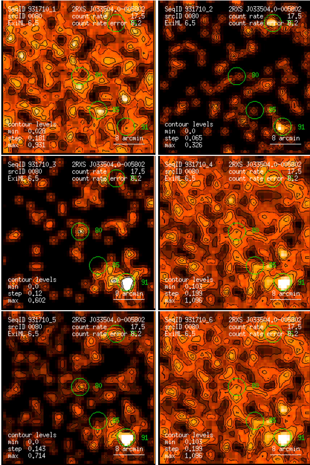
Figure 80: RASS 931710: detection 0080: band rate images, Gaussian filter: (1) PSPC channels 11 – 41, (2) 52 – 90, (3) 91 – 201, (4) 11 – 235, (5) 52 – 201, (6) 11 – 201. Broad band rates in counts/ks. Band rate contour levels in counts/ks/arcmin 2 .
