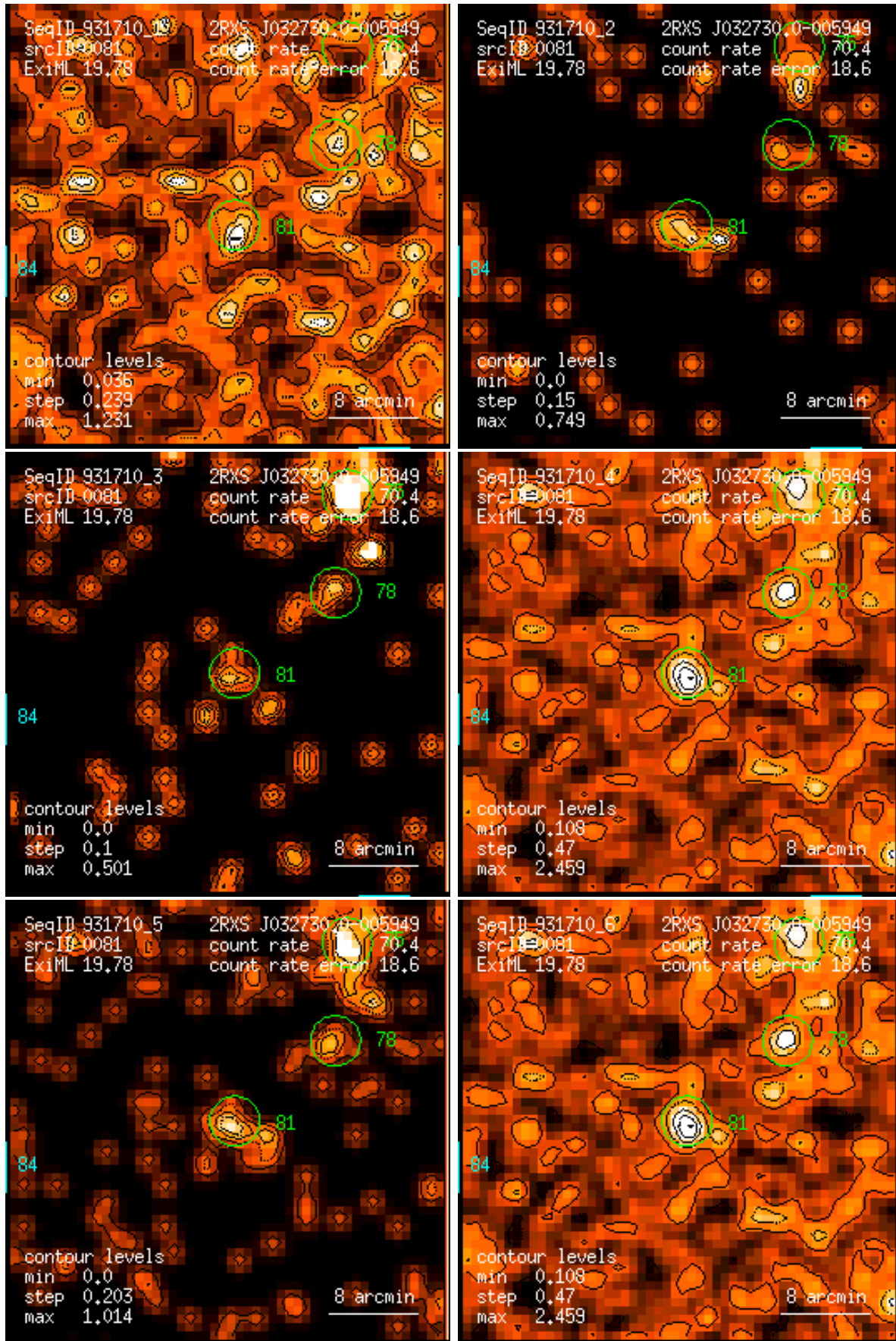
Figure 81: RASS 931710: detection 0081: band rate images, Gaussian filter: (1) PSPC channels 11 – 41, (2) 52 – 90, (3) 91 – 201, (4) 11 – 235, (5) 52 – 201, (6) 11 – 201. Broad band rates in counts/ks. Band rate contour levels in counts/ks/arcmin 2 .
