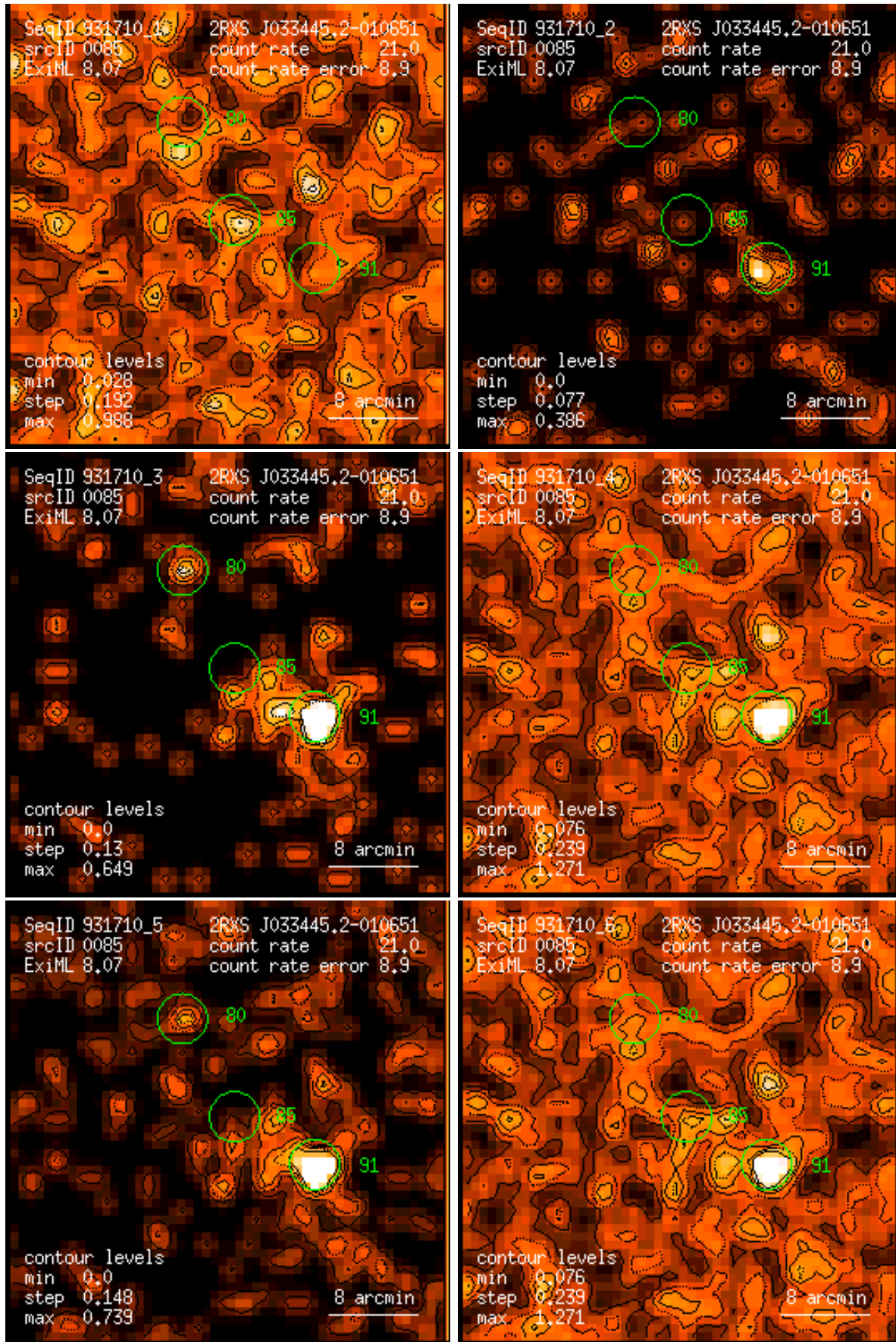
Figure 85: RASS 931710: detection 0085: band rate images, Gaussian filter: (1) PSPC channels 11 – 41, (2) 52 – 90, (3) 91 – 201, (4) 11 – 235, (5) 52 – 201, (6) 11 – 201. Broad band rates in counts/ks. Band rate contour levels in counts/ks/arcmin 2 .
