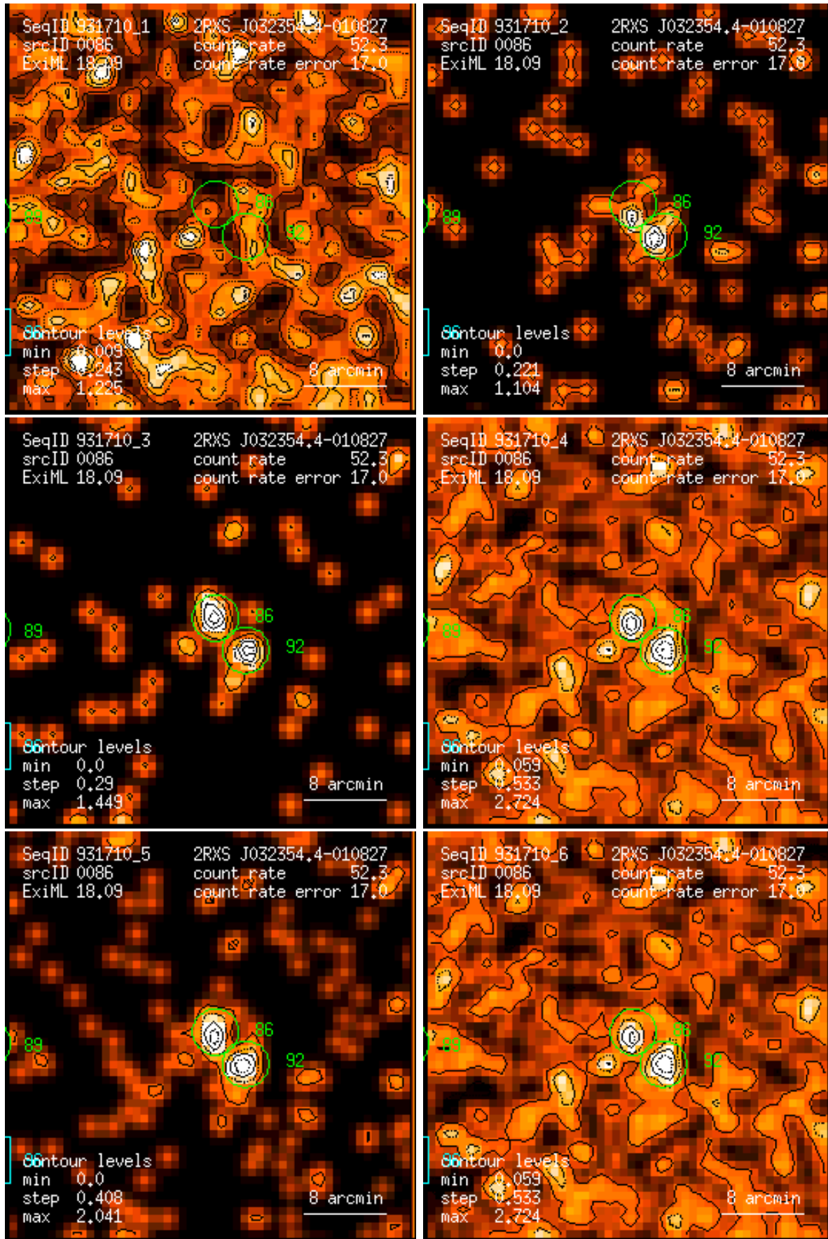
Figure 86: RASS 931710: detection 0086: band rate images, Gaussian filter: (1) PSPC channels 11 – 41, (2) 52 – 90, (3) 91 – 201, (4) 11 – 235, (5) 52 – 201, (6) 11 – 201. Broad band rates in counts/ks. Band rate contour levels in counts/ks/arcmin 2 .
