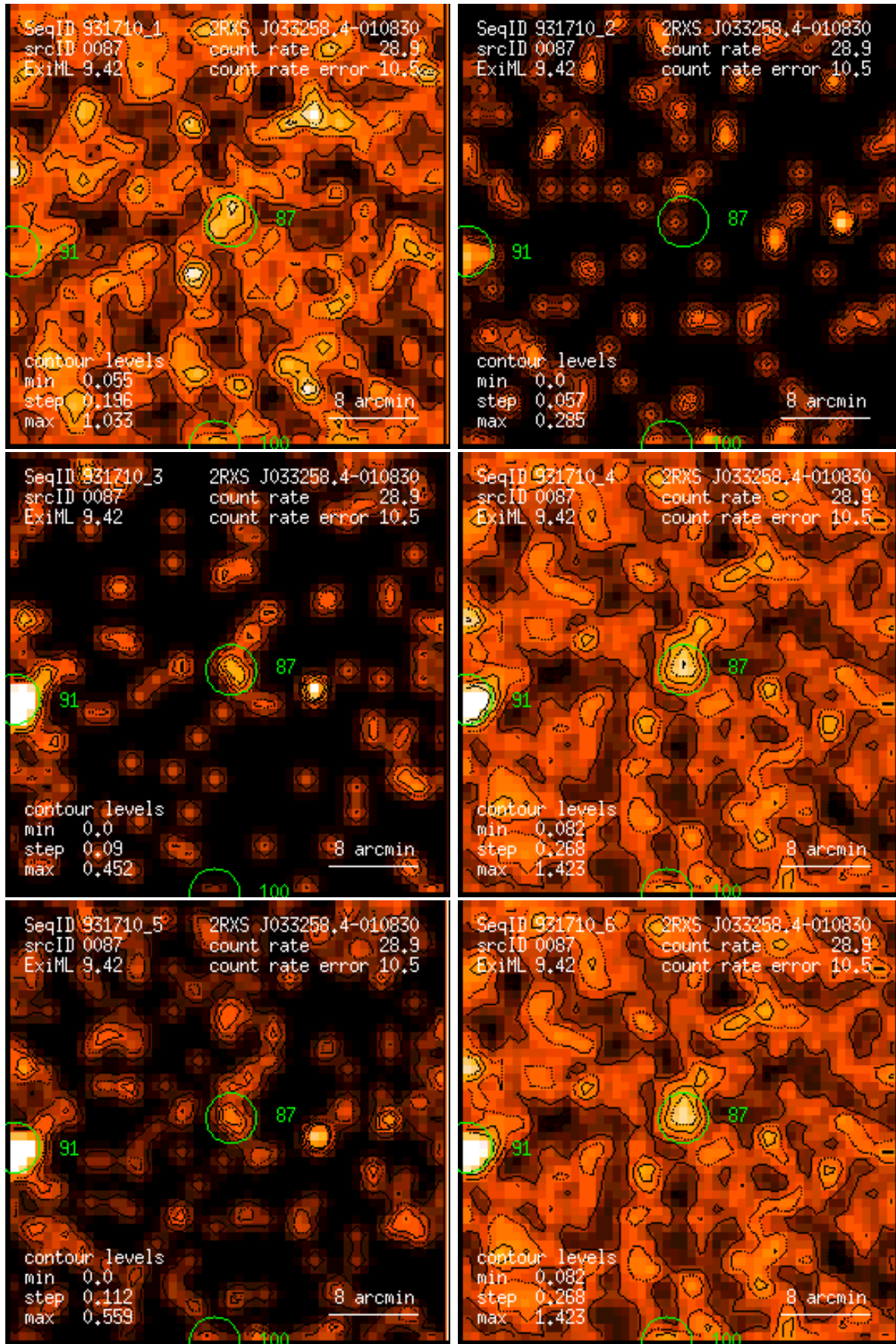
Figure 87: RASS 931710: detection 0087: band rate images, Gaussian filter: (1) PSPC channels 11 – 41, (2) 52 – 90, (3) 91 – 201, (4) 11 – 235, (5) 52 – 201, (6) 11 – 201. Broad band rates in counts/ks. Band rate contour levels in counts/ks/arcmin 2 .
