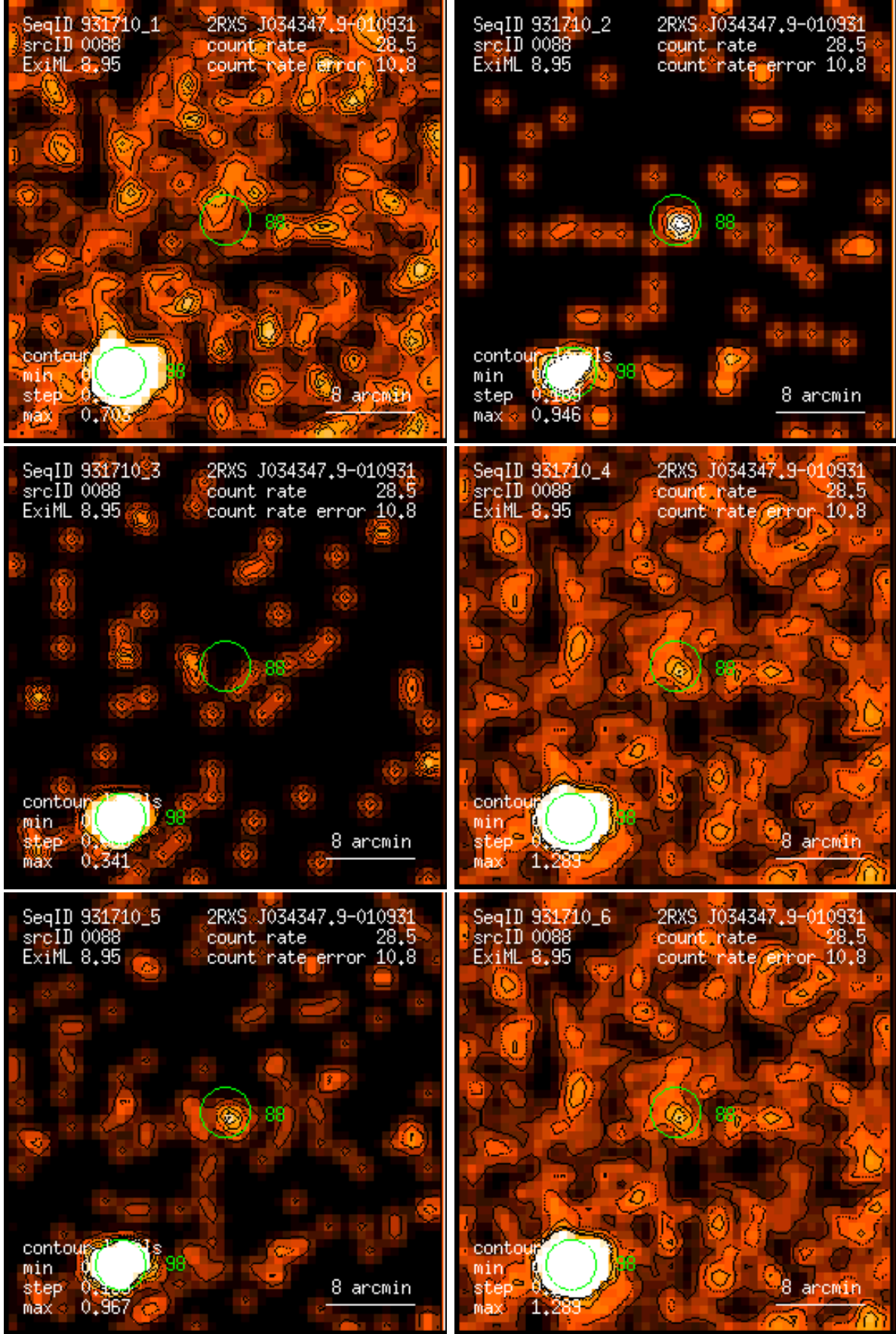
Figure 88: RASS 931710: detection 0088: band rate images, Gaussian filter: (1) PSPC channels 11 – 41, (2) 52 – 90, (3) 91 – 201, (4) 11 – 235, (5) 52 – 201, (6) 11 – 201. Broad band rates in counts/ks. Band rate contour levels in counts/ks/arcmin 2 .
