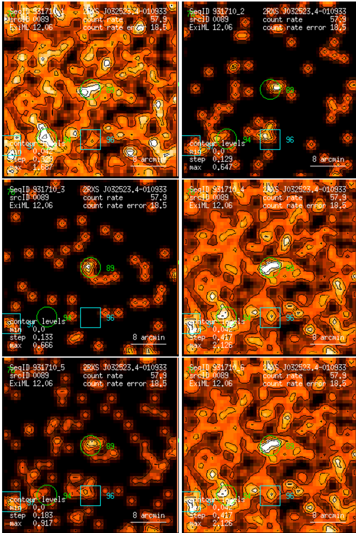
Figure 89: RASS 931710: detection 0089: band rate images, Gaussian filter: (1) PSPC channels 11 – 41, (2) 52 – 90, (3) 91 – 201, (4) 11 – 235, (5) 52 – 201, (6) 11 – 201. Broad band rates in counts/ks. Band rate contour levels in counts/ks/arcmin 2 .
