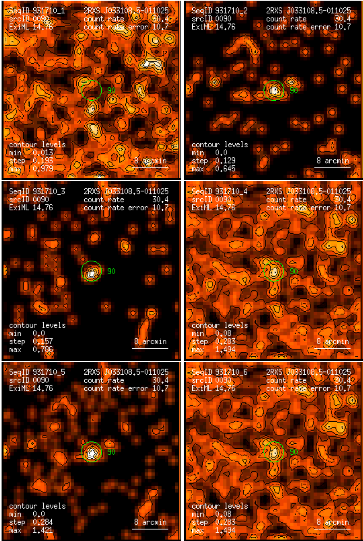
Figure 90: RASS 931710: detection 0090: band rate images, Gaussian filter: (1) PSPC channels 11 – 41, (2) 52 – 90, (3) 91 – 201, (4) 11 – 235, (5) 52 – 201, (6) 11 – 201. Broad band rates in counts/ks. Band rate contour levels in counts/ks/arcmin 2 .
