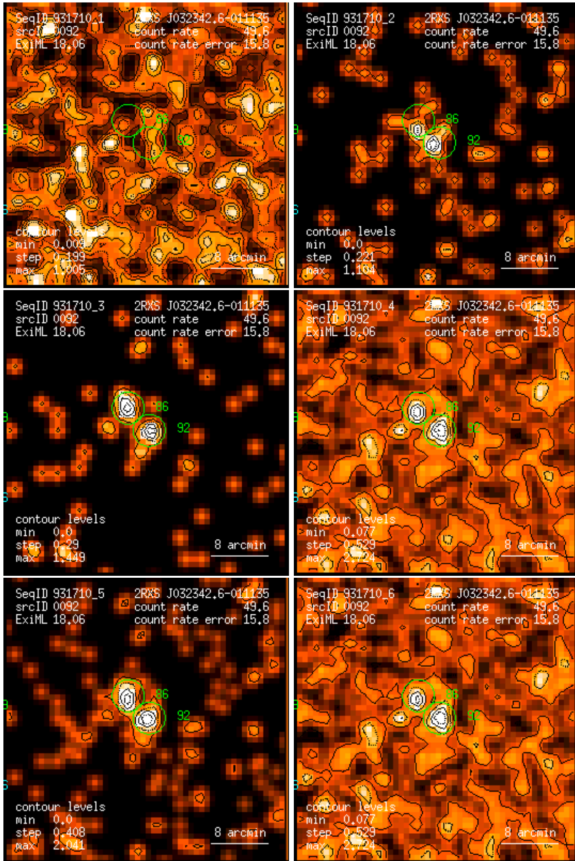
Figure 92: RASS 931710: detection 0092: band rate images, Gaussian filter: (1) PSPC channels 11 – 41, (2) 52 – 90, (3) 91 – 201, (4) 11 – 235, (5) 52 – 201, (6) 11 – 201. Broad band rates in counts/ks. Band rate contour levels in counts/ks/arcmin 2 .
