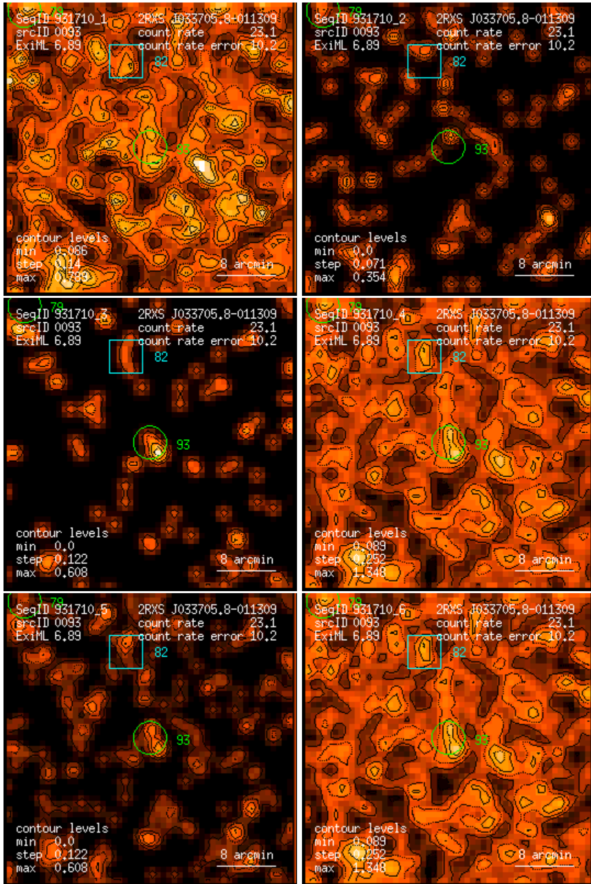
Figure 93: RASS 931710: detection 0093: band rate images, Gaussian filter: (1) PSPC channels 11 – 41, (2) 52 – 90, (3) 91 – 201, (4) 11 – 235, (5) 52 – 201, (6) 11 – 201. Broad band rates in counts/ks. Band rate contour levels in counts/ks/arcmin 2 .
