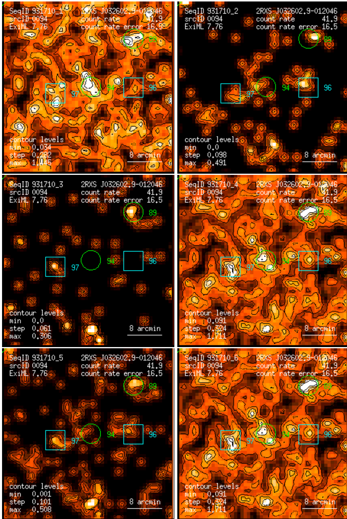
Figure 94: RASS 931710: detection 0094: band rate images, Gaussian filter: (1) PSPC channels 11 – 41, (2) 52 – 90, (3) 91 – 201, (4) 11 – 235, (5) 52 – 201, (6) 11 – 201. Broad band rates in counts/ks. Band rate contour levels in counts/ks/arcmin 2 .
