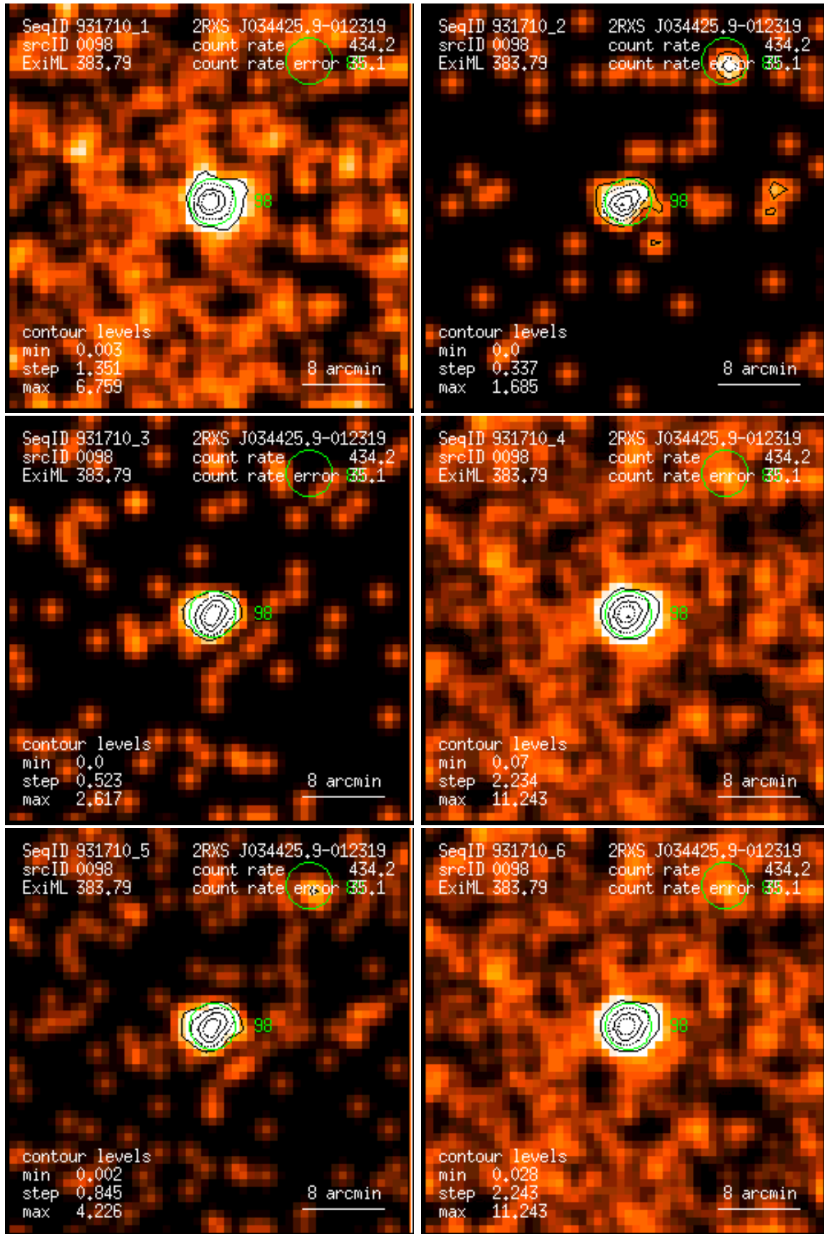
Figure 98: RASS 931710: detection 0098: band rate images, Gaussian filter: (1) PSPC channels 11 – 41, (2) 52 – 90, (3) 91 – 201, (4) 11 – 235, (5) 52 – 201, (6) 11 – 201. Broad band rates in counts/ks. Band rate contour levels in counts/ks/arcmin 2 .
