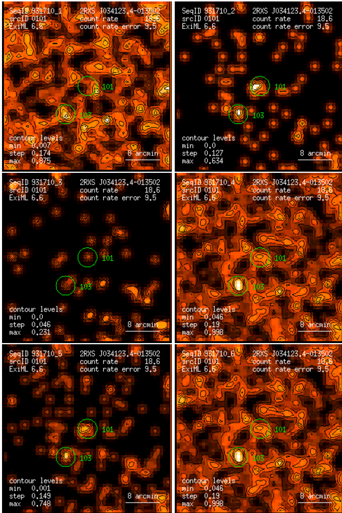
Figure 101: RASS 931710: detection 0101: band rate images, Gaussian filter: (1) PSPC channels 11 – 41, (2) 52 – 90, (3) 91 – 201, (4) 11 – 235, (5) 52 – 201, (6) 11 – 201. Broad band rates in counts/ks. Band rate contour levels in counts/ks/arcmin 2 .
