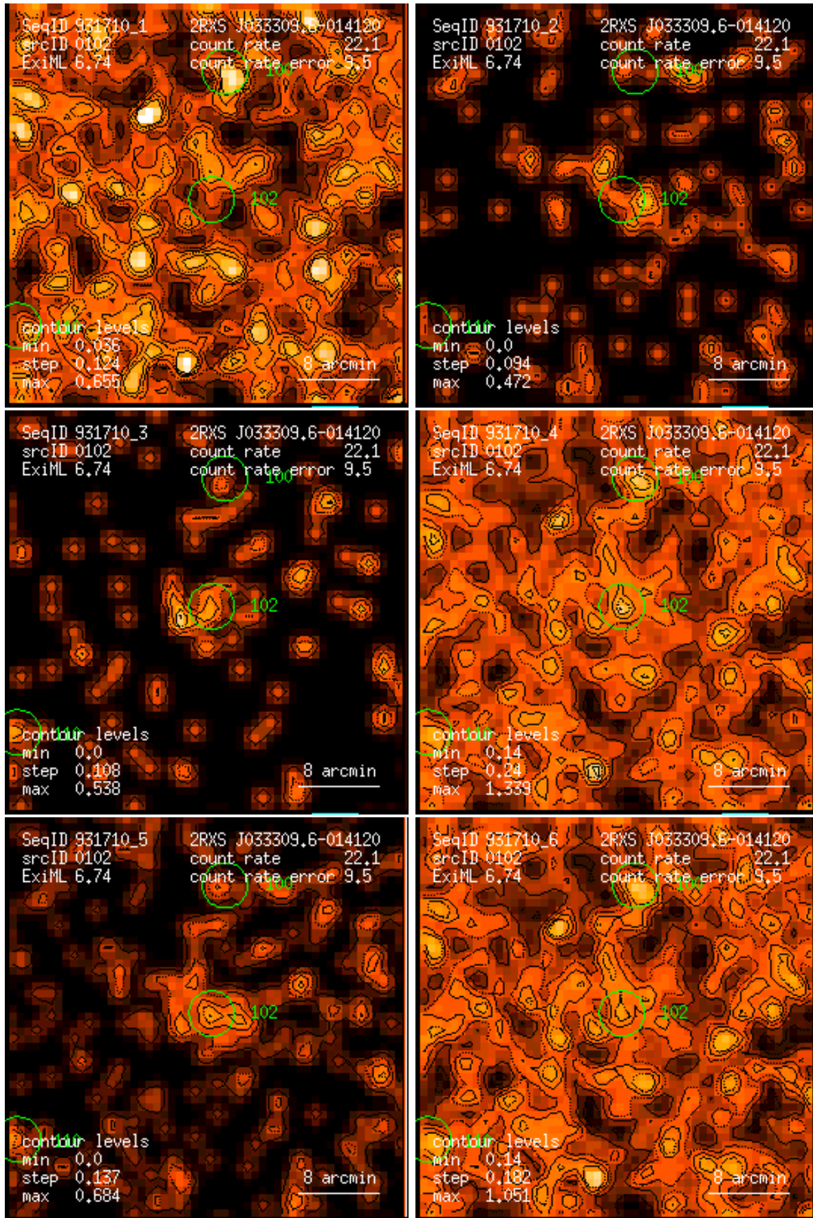
Figure 102: RASS 931710: detection 0102: band rate images, Gaussian filter: (1) PSPC channels 11 – 41, (2) 52 – 90, (3) 91 – 201, (4) 11 – 235, (5) 52 – 201, (6) 11 – 201. Broad band rates in counts/ks. Band rate contour levels in counts/ks/arcmin 2 .
