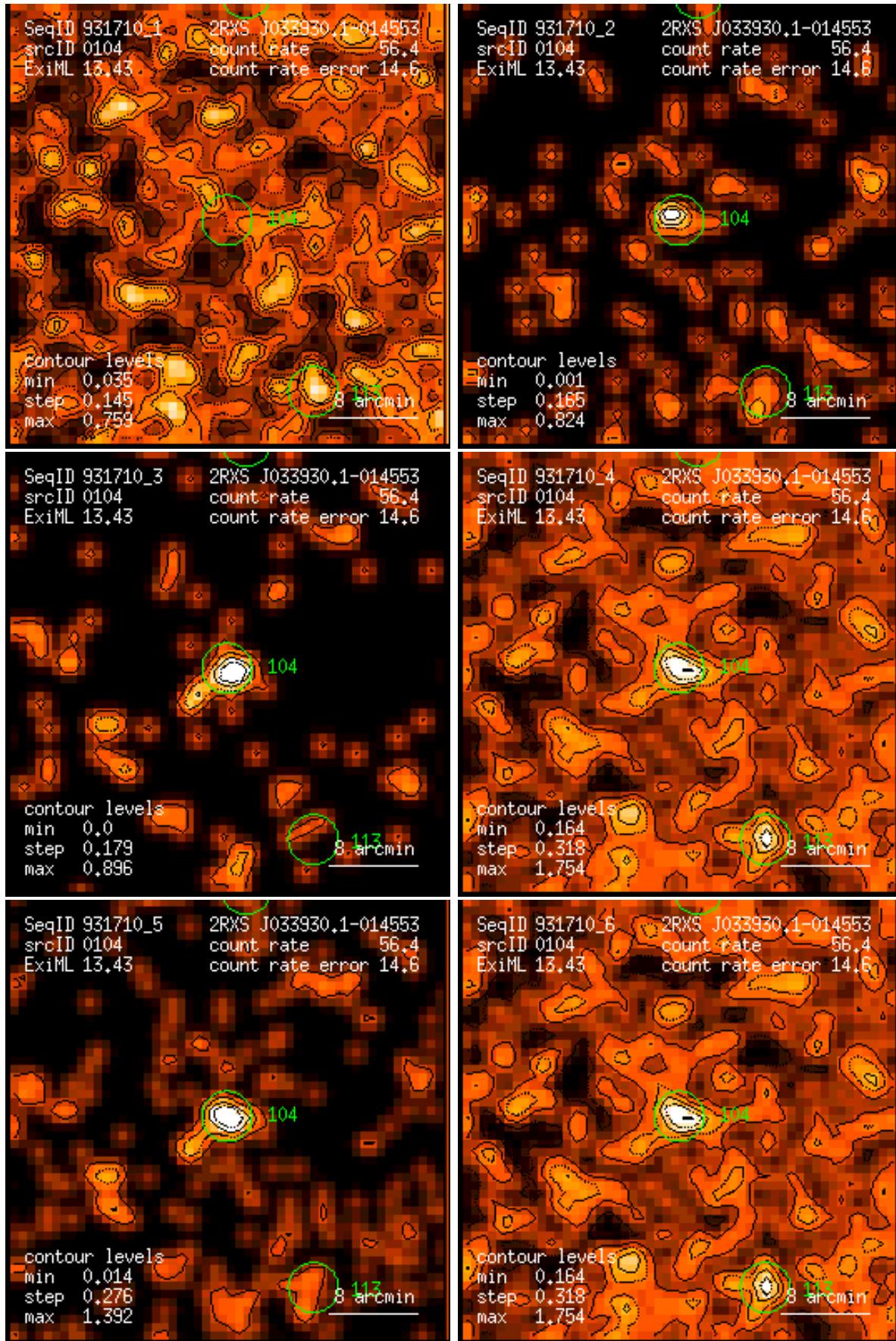
Figure 104: RASS 931710: detection 0104: band rate images, Gaussian filter: (1) PSPC channels 11 – 41, (2) 52 – 90, (3) 91 – 201, (4) 11 – 235, (5) 52 – 201, (6) 11 – 201. Broad band rates in counts/ks. Band rate contour levels in counts/ks/arcmin 2 .
