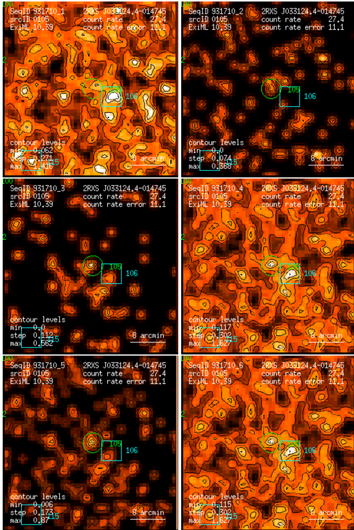
Figure 105: RASS 931710: detection 0105: band rate images, Gaussian filter: (1) PSPC channels 11 – 41, (2) 52 – 90, (3) 91 – 201, (4) 11 – 235, (5) 52 – 201, (6) 11 – 201. Broad band rates in counts/ks. Band rate contour levels in counts/ks/arcmin 2 .
