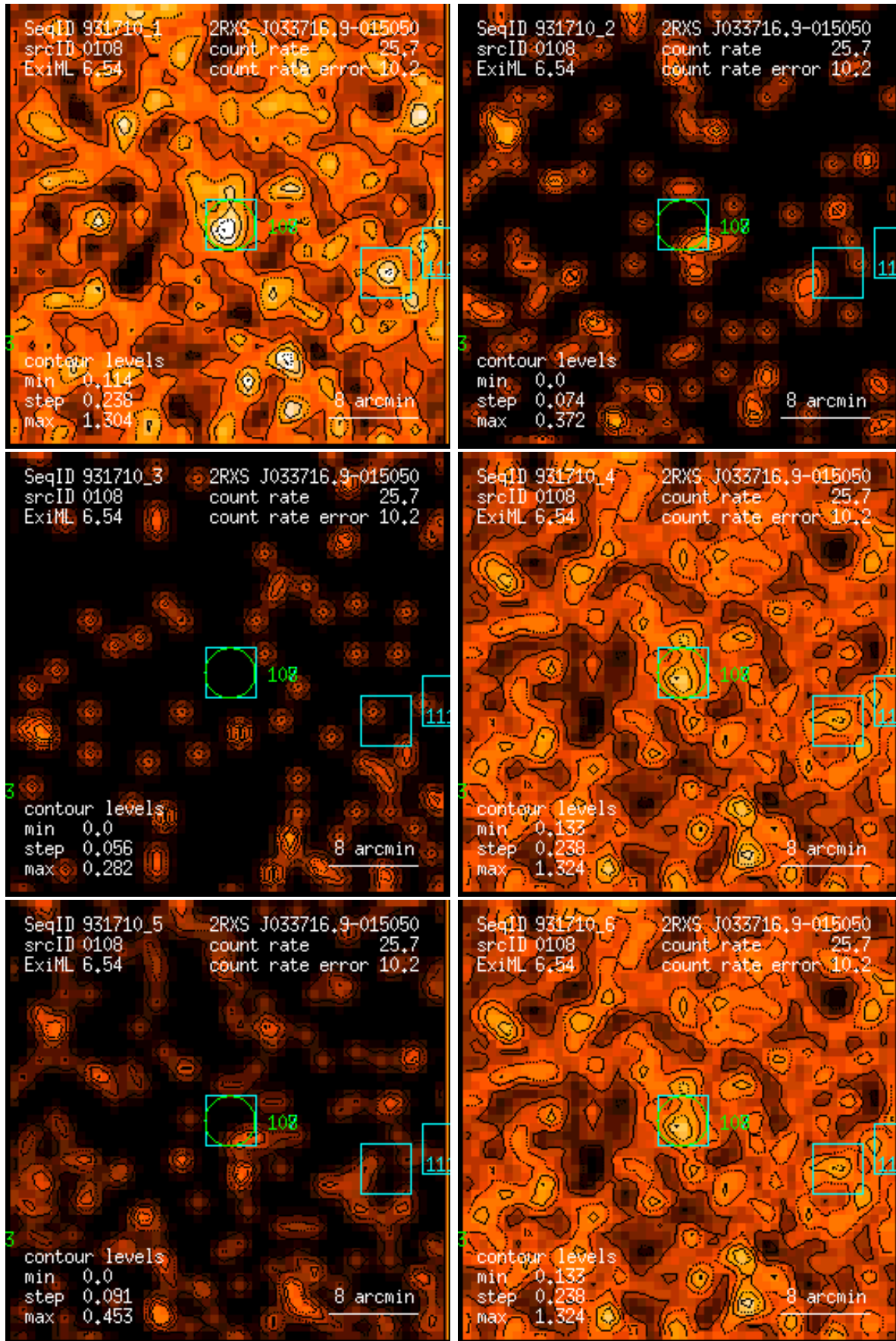
Figure 108: RASS 931710: detection 0108: band rate images, Gaussian filter: (1) PSPC channels 11 – 41, (2) 52 – 90, (3) 91 – 201, (4) 11 – 235, (5) 52 – 201, (6) 11 – 201. Broad band rates in counts/ks. Band rate contour levels in counts/ks/arcmin 2 .
