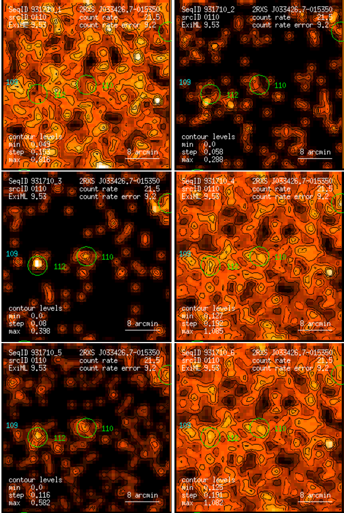
Figure 110: RASS 931710: detection 0110: band rate images, Gaussian filter: (1) PSPC channels 11 – 41, (2) 52 – 90, (3) 91 – 201, (4) 11 – 235, (5) 52 – 201, (6) 11 – 201. Broad band rates in counts/ks. Band rate contour levels in counts/ks/arcmin 2 .
