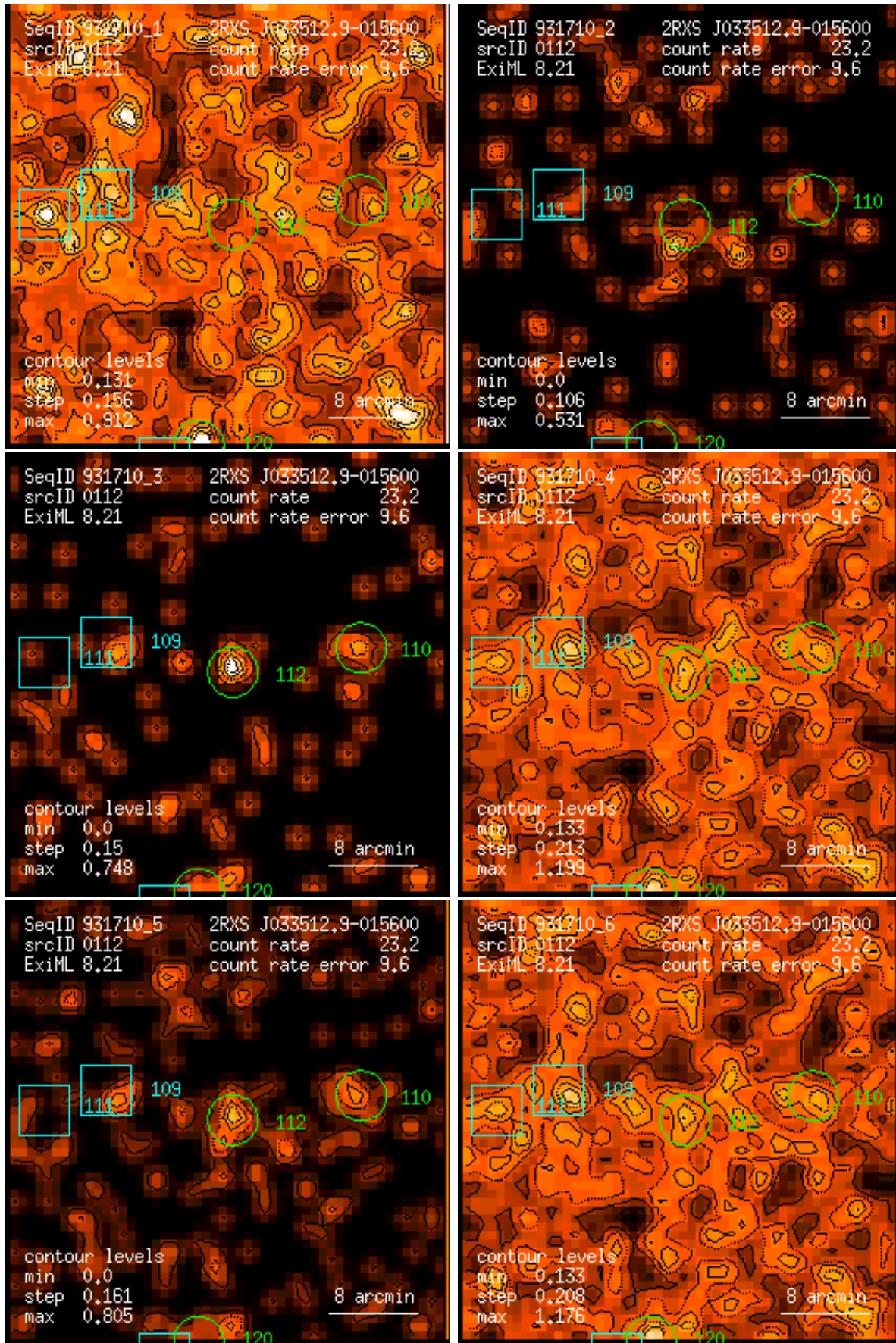
Figure 112: RASS 931710: detection 0112: band rate images, Gaussian filter: (1) PSPC channels 11 – 41, (2) 52 – 90, (3) 91 – 201, (4) 11 – 235, (5) 52 – 201, (6) 11 – 201. Broad band rates in counts/ks. Band rate contour levels in counts/ks/arcmin 2 .
