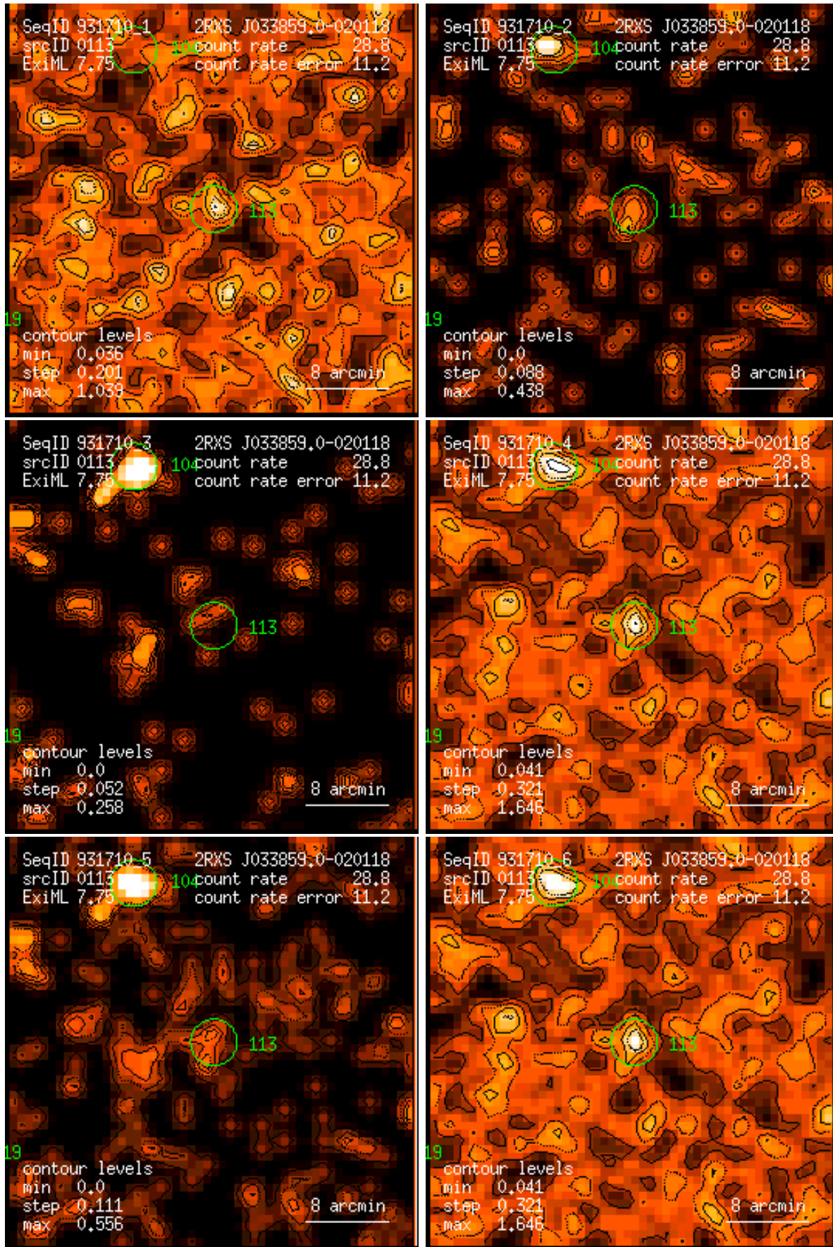
Figure 113: RASS 931710: detection 0113: band rate images, Gaussian filter: (1) PSPC channels 11 – 41, (2) 52 – 90, (3) 91 – 201, (4) 11 – 235, (5) 52 – 201, (6) 11 – 201. Broad band rates in counts/ks. Band rate contour levels in counts/ks/arcmin 2 .
