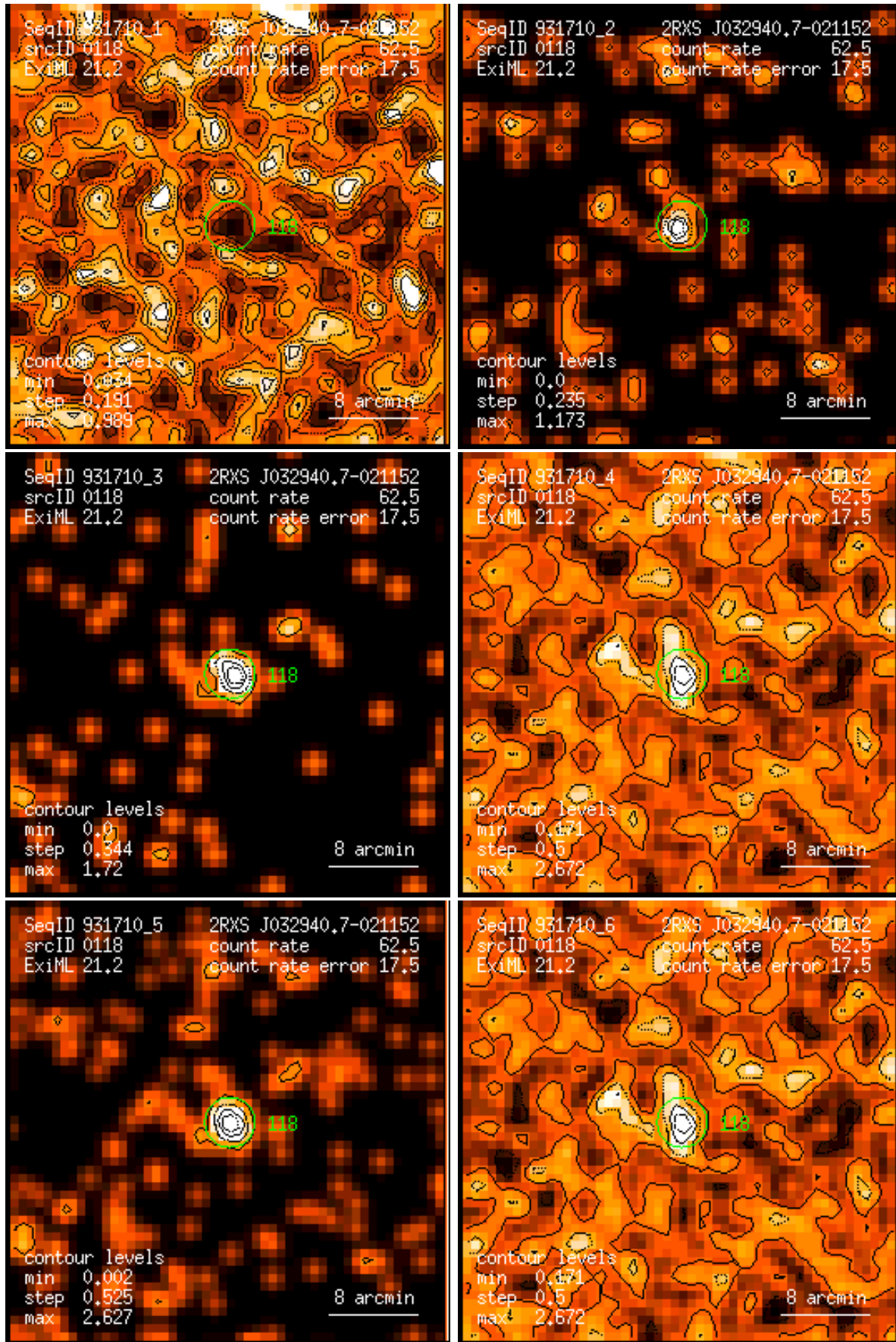
Figure 118: RASS 931710: detection 0118: band rate images, Gaussian filter: (1) PSPC channels 11 – 41, (2) 52 – 90, (3) 91 – 201, (4) 11 – 235, (5) 52 – 201, (6) 11 – 201. Broad band rates in counts/ks. Band rate contour levels in counts/ks/arcmin 2 .
