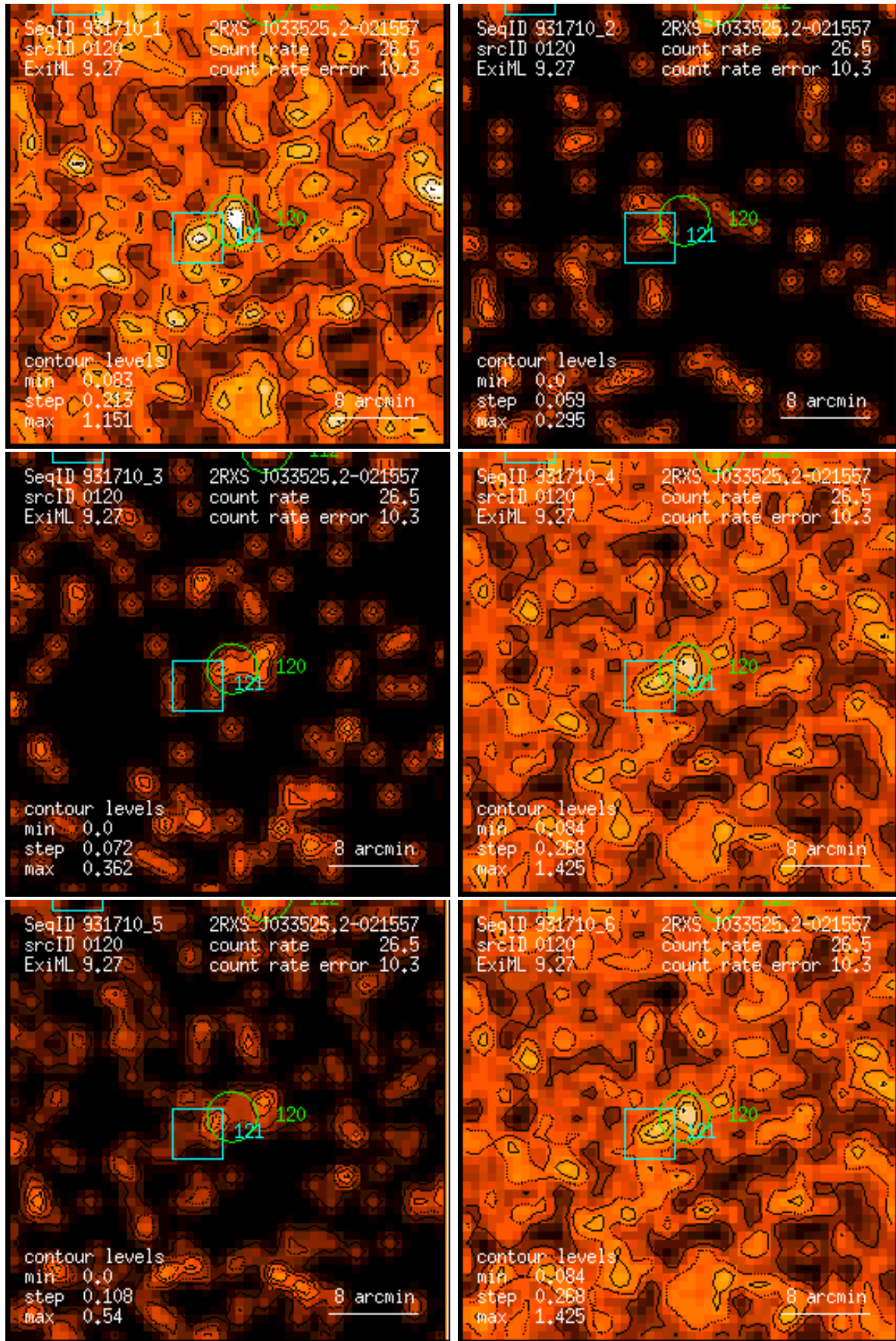
Figure 120: RASS 931710: detection 0120: band rate images, Gaussian filter: (1) PSPC channels 11 – 41, (2) 52 – 90, (3) 91 – 201, (4) 11 – 235, (5) 52 – 201, (6) 11 – 201. Broad band rates in counts/ks. Band rate contour levels in counts/ks/arcmin 2 .
