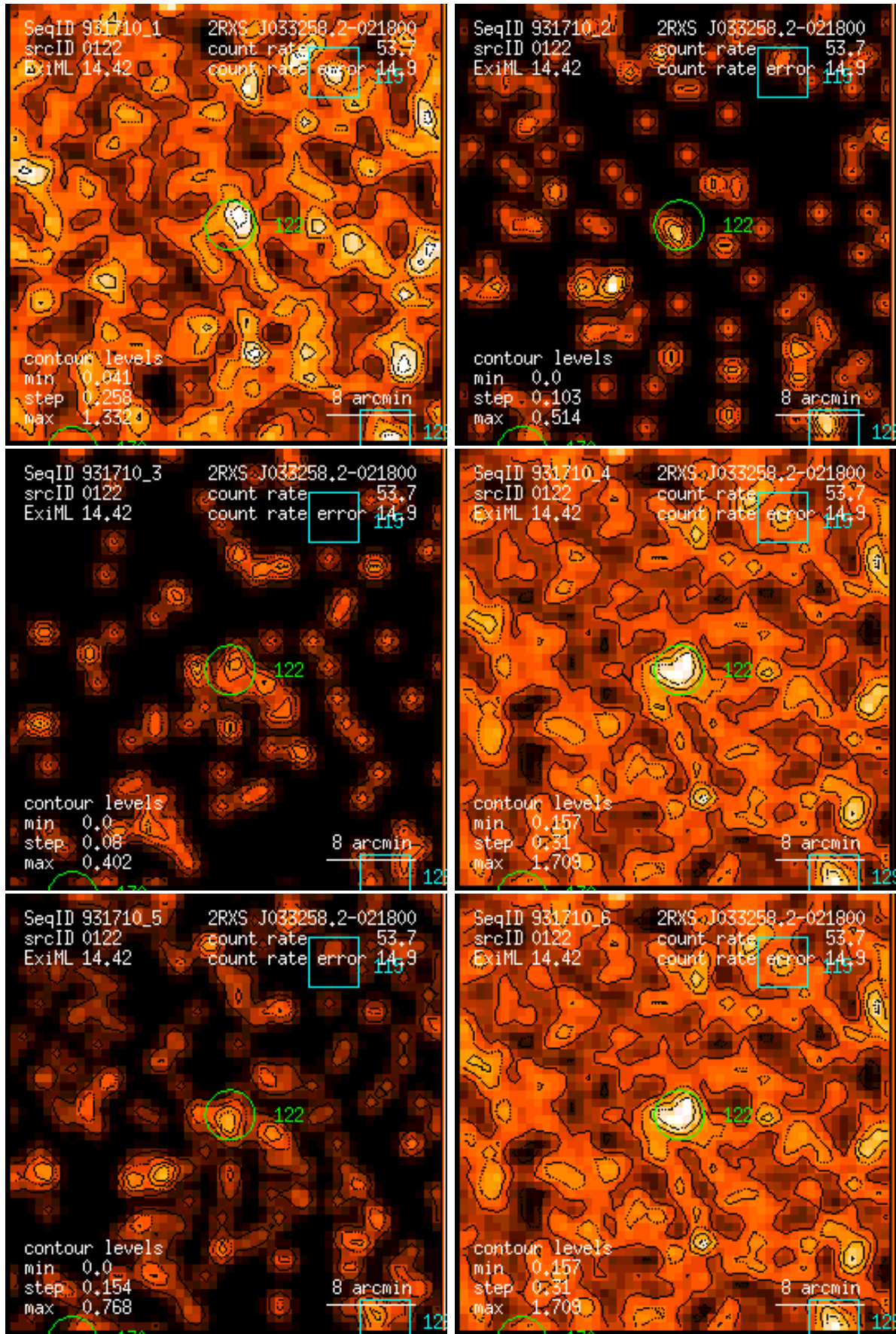
Figure 122: RASS 931710: detection 0122: band rate images, Gaussian filter: (1) PSPC channels 11 – 41, (2) 52 – 90, (3) 91 – 201, (4) 11 – 235, (5) 52 – 201, (6) 11 – 201. Broad band rates in counts/ks. Band rate contour levels in counts/ks/arcmin 2 .
