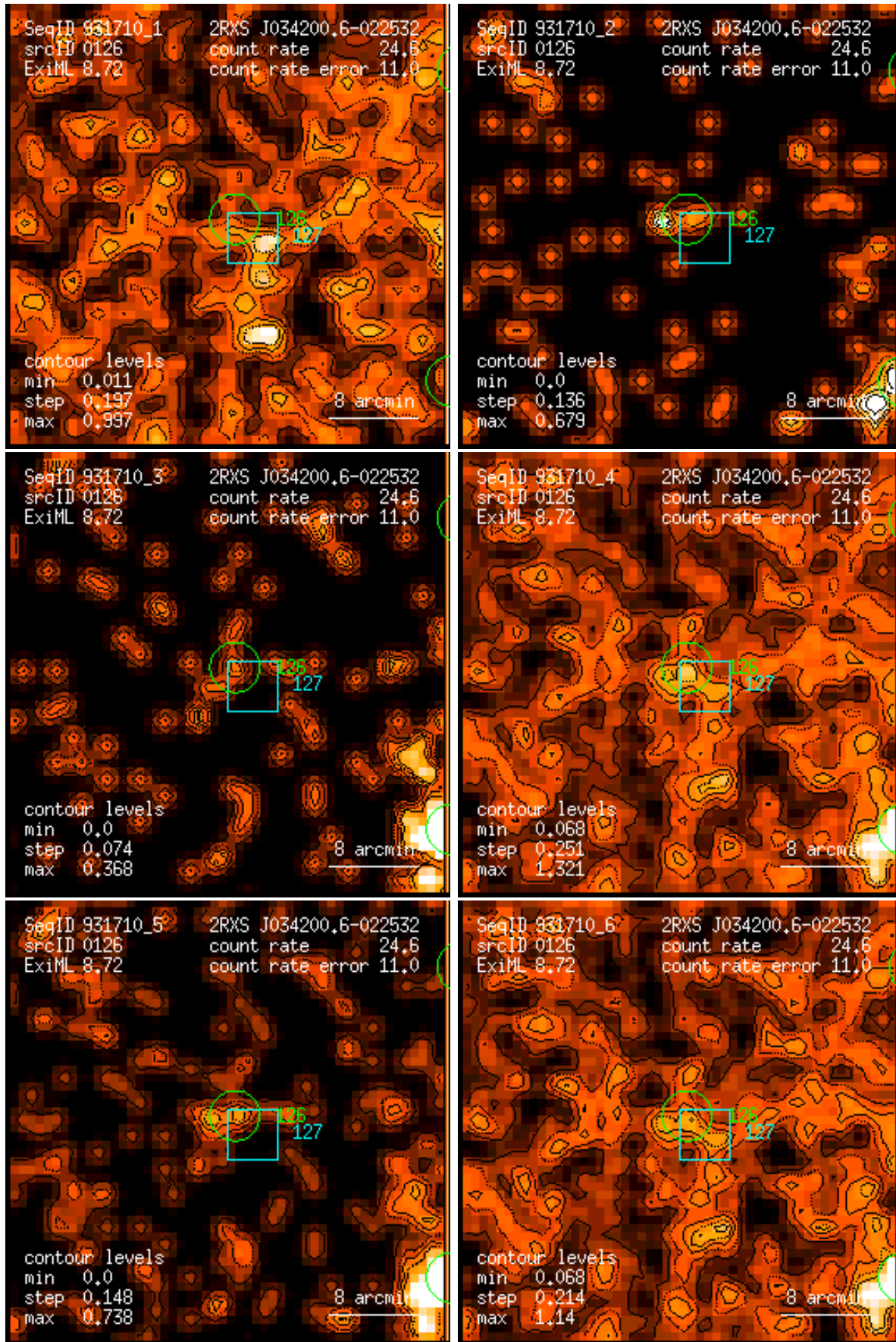
Figure 126: RASS 931710: detection 0126: band rate images, Gaussian filter: (1) PSPC channels 11 – 41, (2) 52 – 90, (3) 91 – 201, (4) 11 – 235, (5) 52 – 201, (6) 11 – 201. Broad band rates in counts/ks. Band rate contour levels in counts/ks/arcmin 2 .
