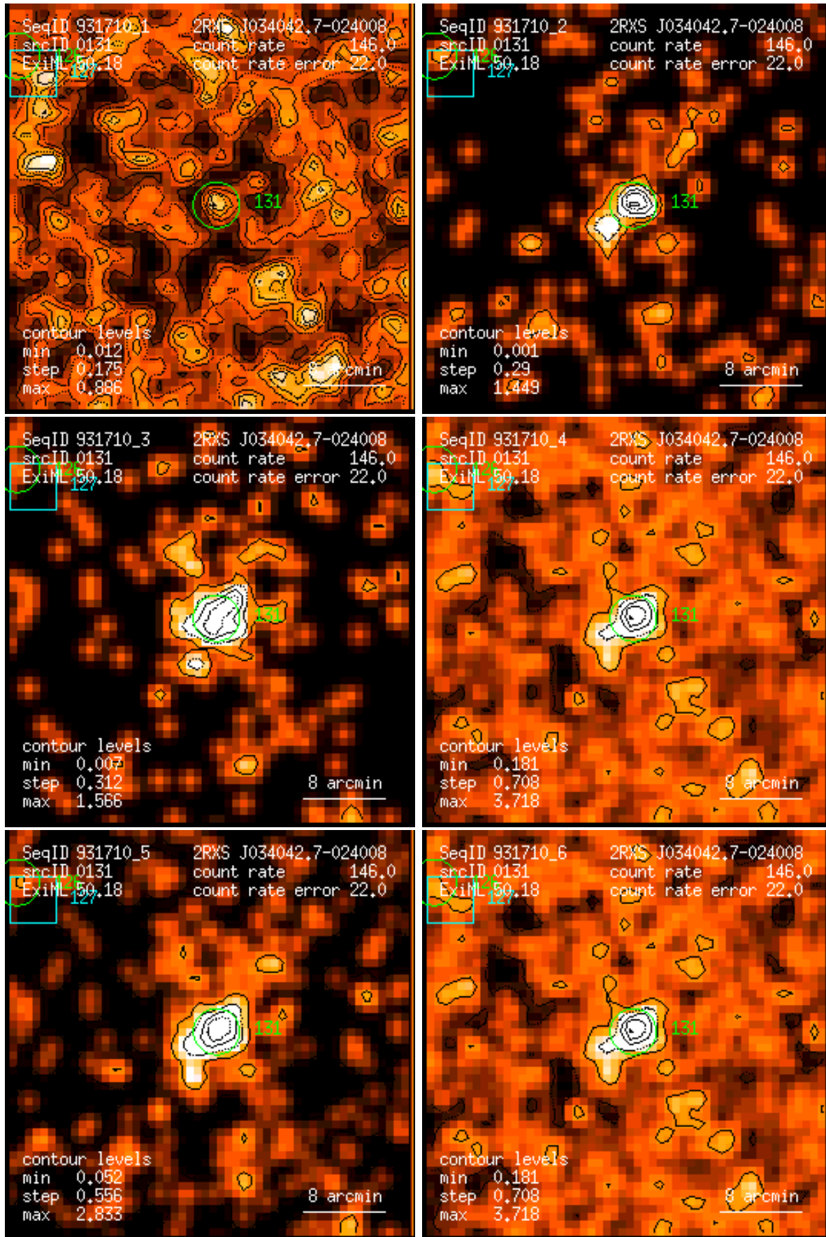
Figure 131: RASS 931710: detection 0131: band rate images, Gaussian filter: (1) PSPC channels 11 – 41, (2) 52 – 90, (3) 91 – 201, (4) 11 – 235, (5) 52 – 201, (6) 11 – 201. Broad band rates in counts/ks. Band rate contour levels in counts/ks/arcmin 2 .
