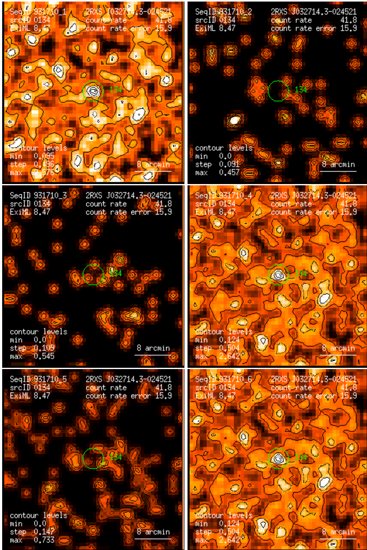
Figure 134: RASS 931710: detection 0134: band rate images, Gaussian filter: (1) PSPC channels 11 – 41, (2) 52 – 90, (3) 91 – 201, (4) 11 – 235, (5) 52 – 201, (6) 11 – 201. Broad band rates in counts/ks. Band rate contour levels in counts/ks/arcmin 2 .
