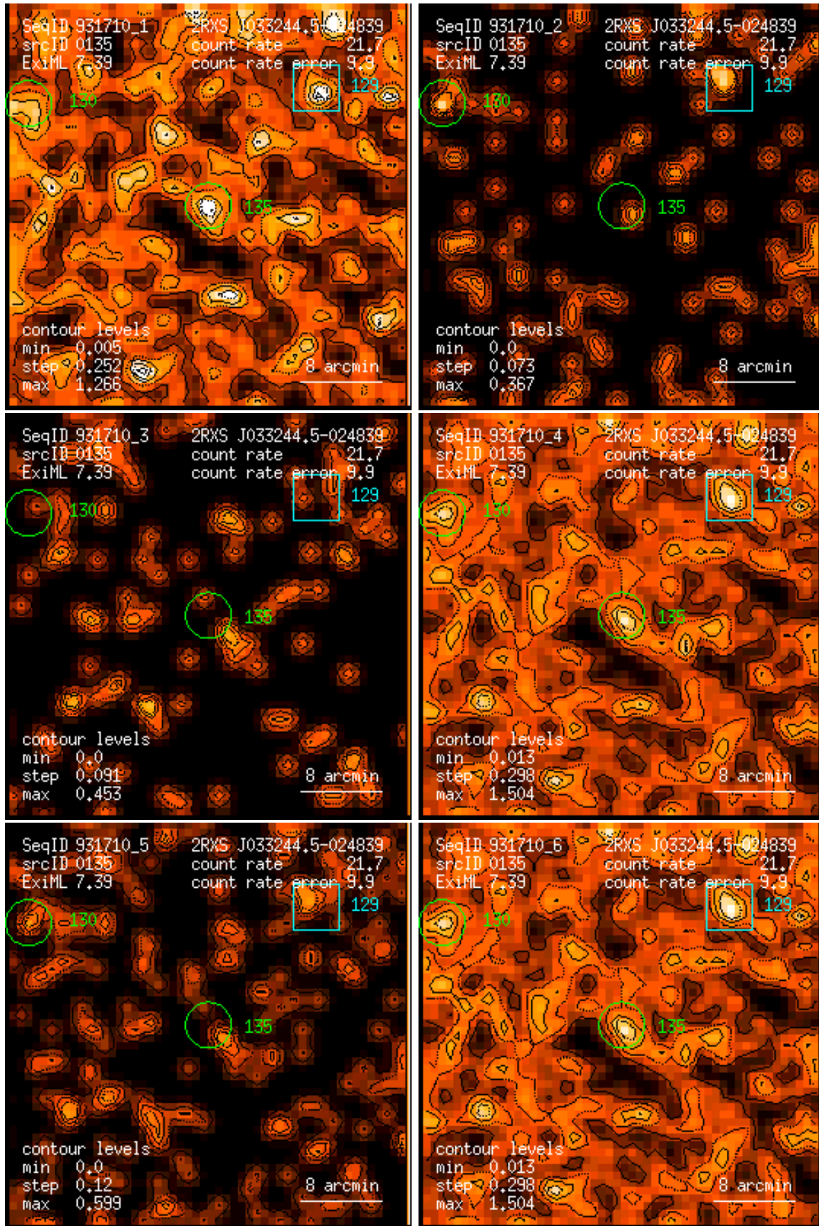
Figure 135: RASS 931710: detection 0135: band rate images, Gaussian filter: (1) PSPC channels 11 – 41, (2) 52 – 90, (3) 91 – 201, (4) 11 – 235, (5) 52 – 201, (6) 11 – 201. Broad band rates in counts/ks. Band rate contour levels in counts/ks/arcmin 2 .
