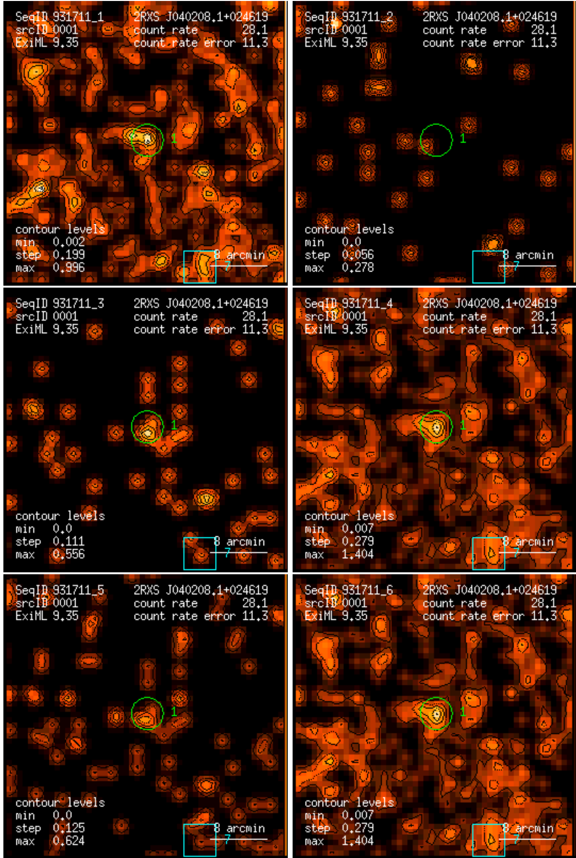
Figure 1: RASS 931711: detection 0001: band rate images, Gaussian filter: (1) PSPC channels 11 – 41, (2) 52 – 90, (3) 91 – 201, (4) 11 – 235, (5) 52 – 201, (6) 11 – 201. Broad band rates in counts/ks. Band rate contour levels in counts/ks/arcmin 2 .
