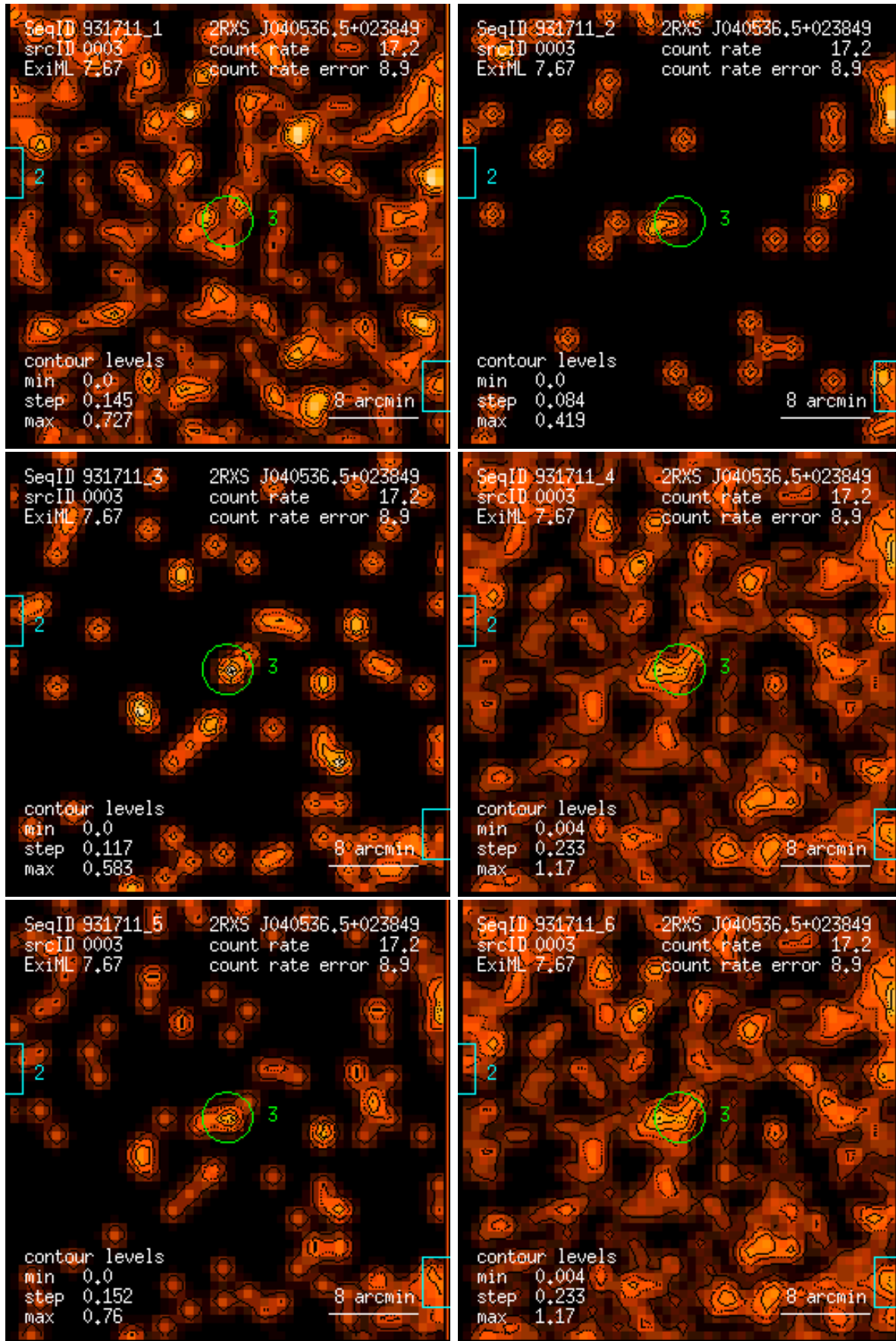
Figure 3: RASS 931711: detection 0003: band rate images, Gaussian filter: (1) PSPC channels 11 – 41, (2) 52 – 90, (3) 91 – 201, (4) 11 – 235, (5) 52 – 201, (6) 11 – 201. Broad band rates in counts/ks. Band rate contour levels in counts/ks/arcmin 2 .
