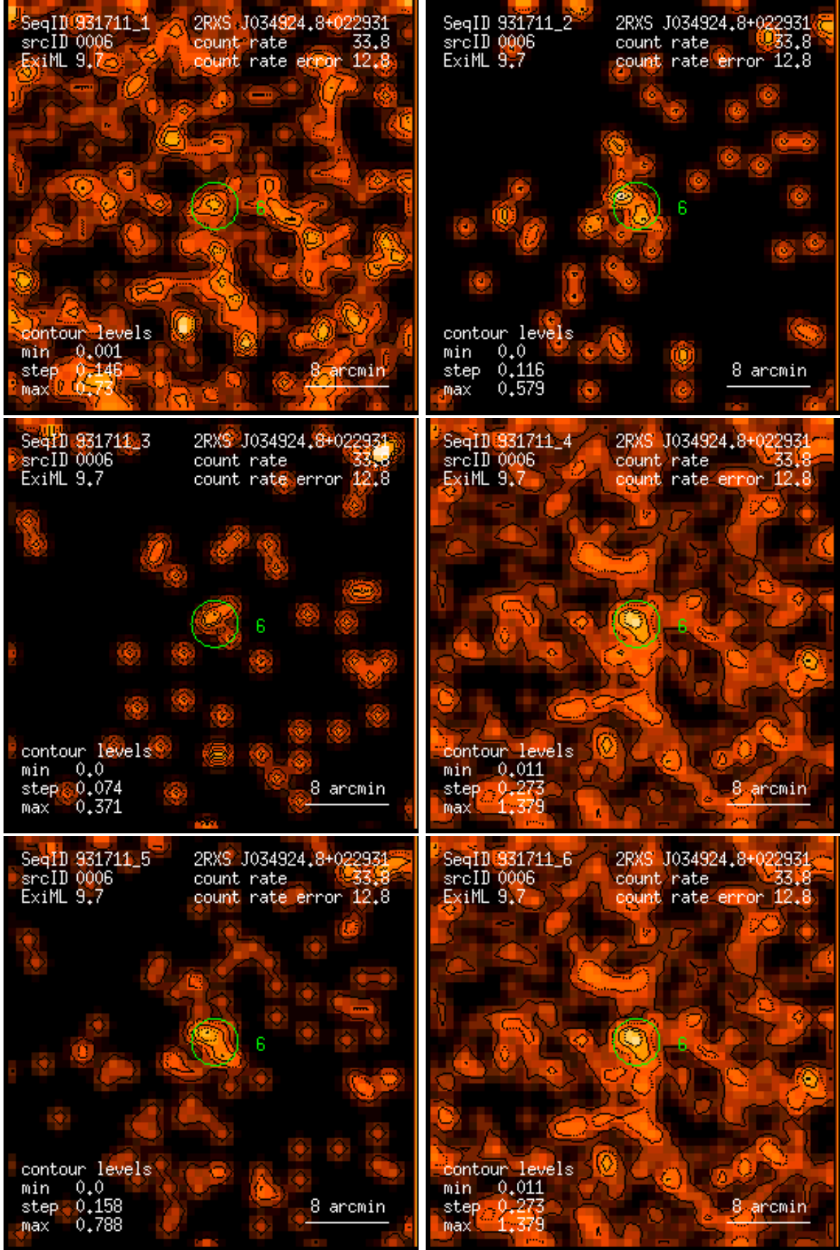
Figure 6: RASS 931711: detection 0006: band rate images, Gaussian filter: (1) PSPC channels 11 – 41, (2) 52 – 90, (3) 91 – 201, (4) 11 – 235, (5) 52 – 201, (6) 11 – 201. Broad band rates in counts/ks. Band rate contour levels in counts/ks/arcmin 2 .
