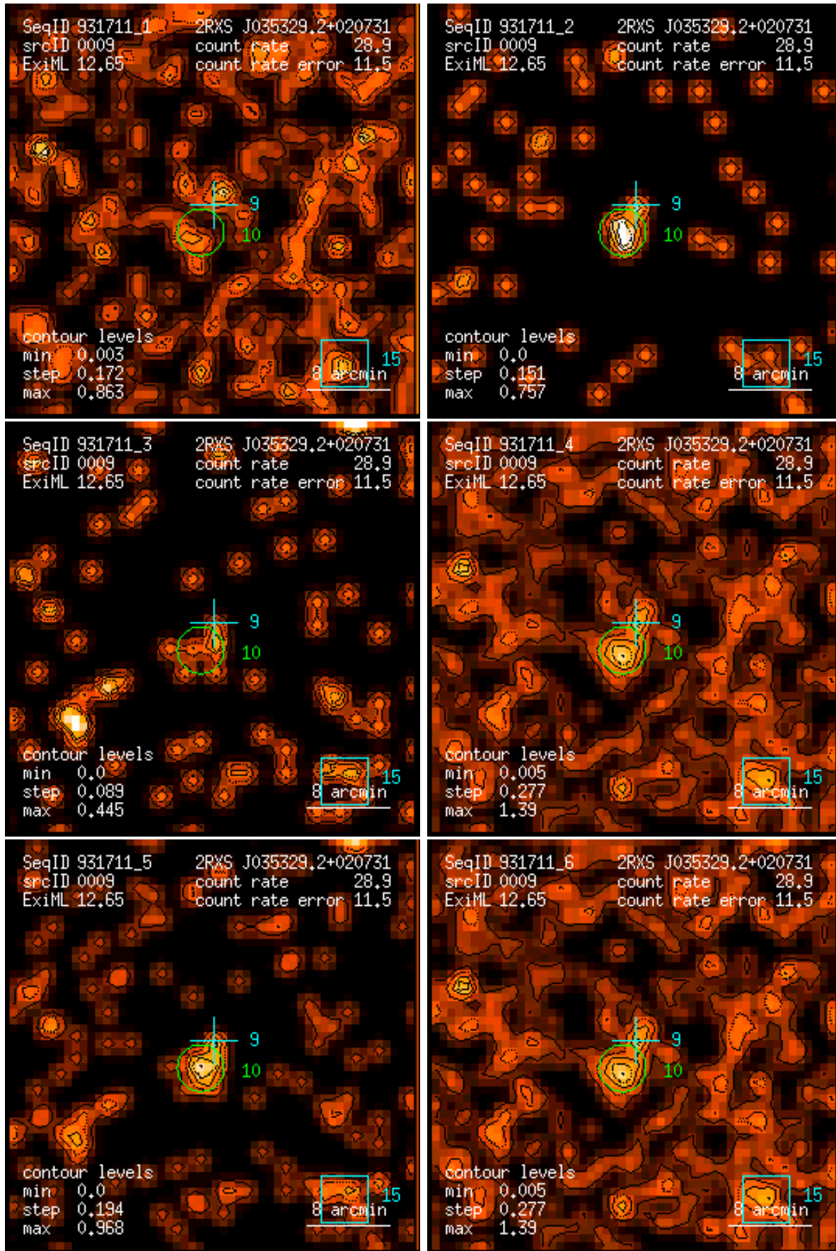
Figure 9: RASS 931711: detection 0009: band rate images, Gaussian filter: (1) PSPC channels 11 – 41, (2) 52 – 90, (3) 91 – 201, (4) 11 – 235, (5) 52 – 201, (6) 11 – 201. Broad band rates in counts/ks. Band rate contour levels in counts/ks/arcmin 2 .
