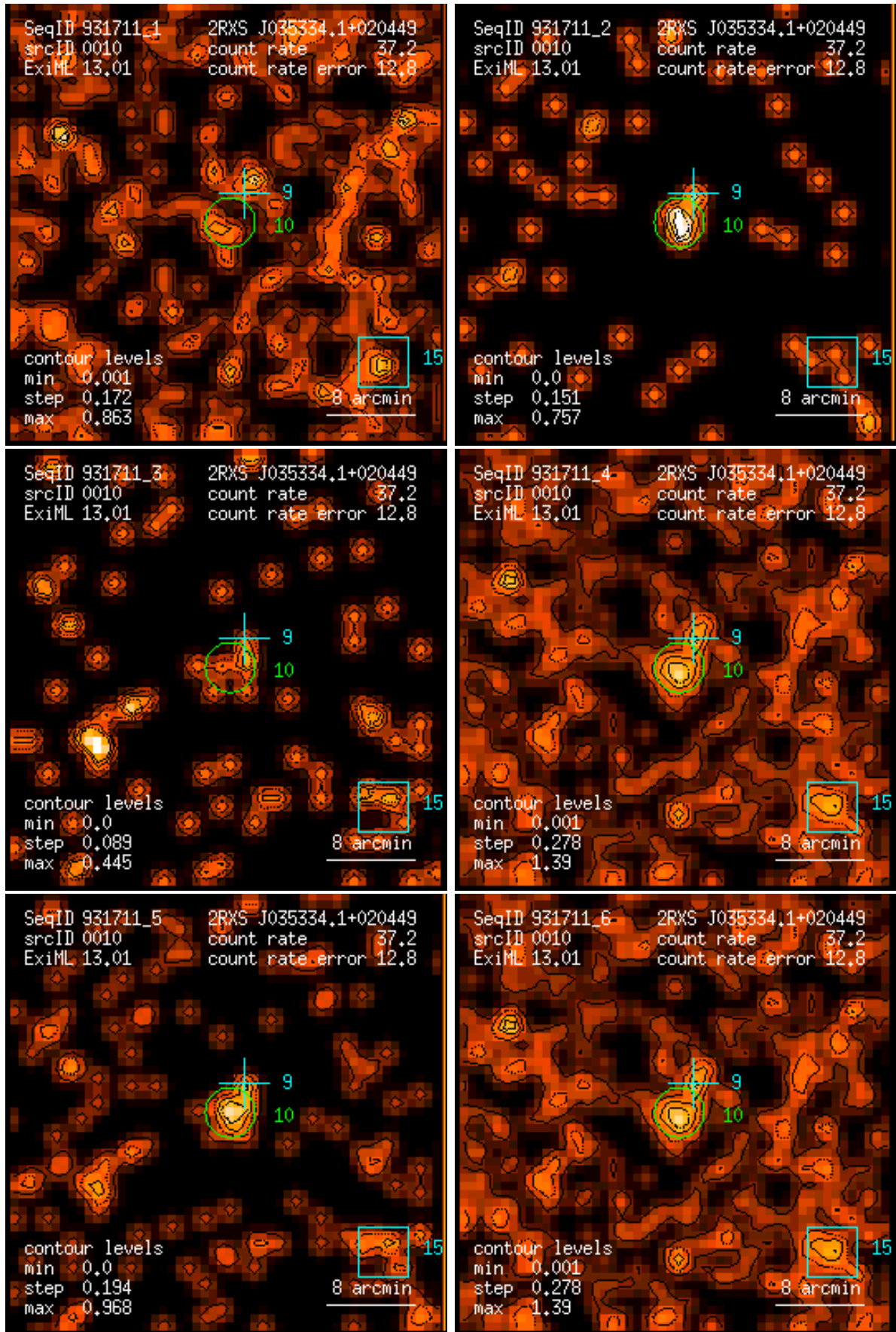
Figure 10: RASS 931711: detection 0010: band rate images, Gaussian filter: (1) PSPC channels 11 – 41, (2) 52 – 90, (3) 91 – 201, (4) 11 – 235, (5) 52 – 201, (6) 11 – 201. Broad band rates in counts/ks. Band rate contour levels in counts/ks/arcmin 2 .
