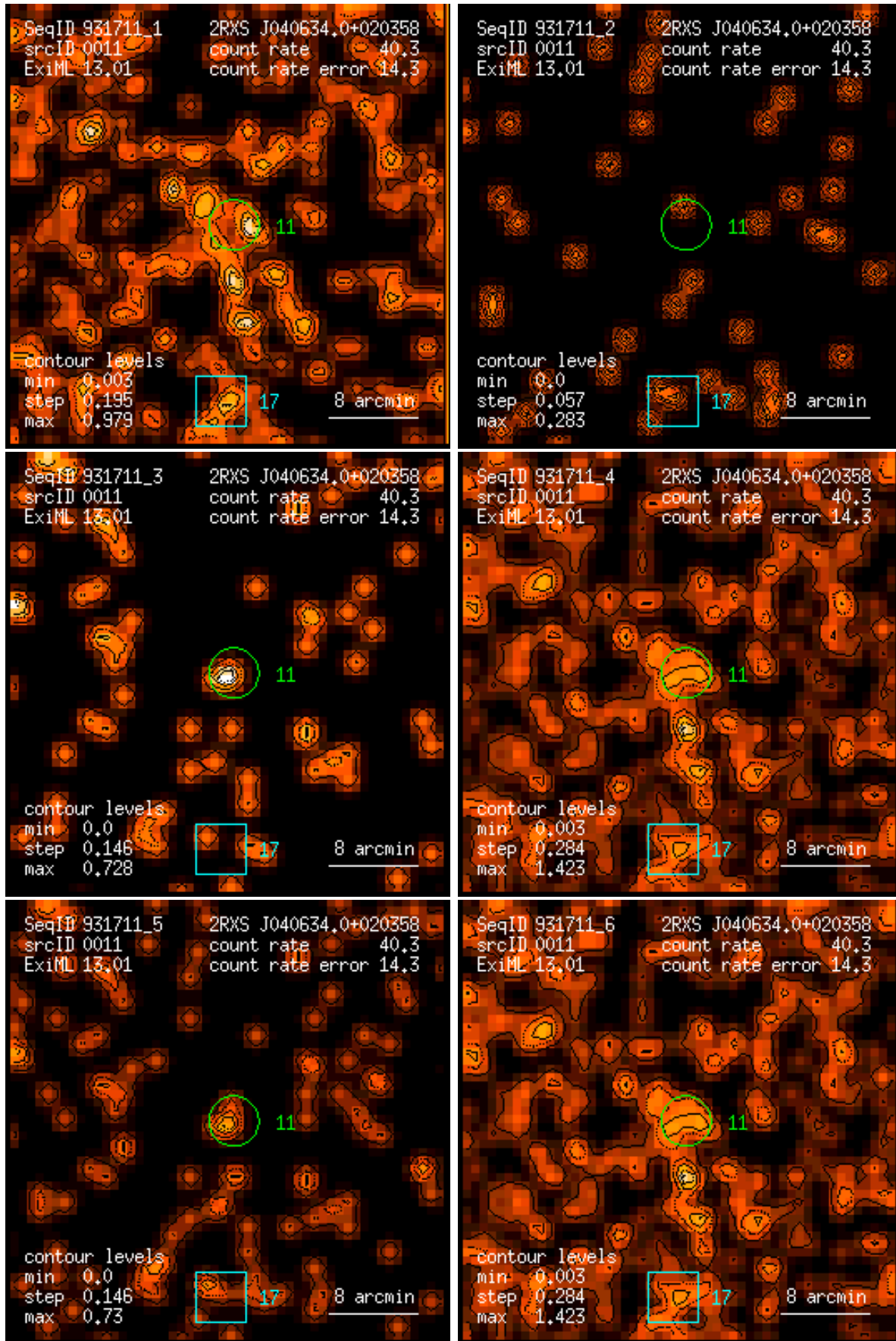
Figure 11: RASS 931711: detection 0011: band rate images, Gaussian filter: (1) PSPC channels 11 – 41, (2) 52 – 90, (3) 91 – 201, (4) 11 – 235, (5) 52 – 201, (6) 11 – 201. Broad band rates in counts/ks. Band rate contour levels in counts/ks/arcmin 2 .
